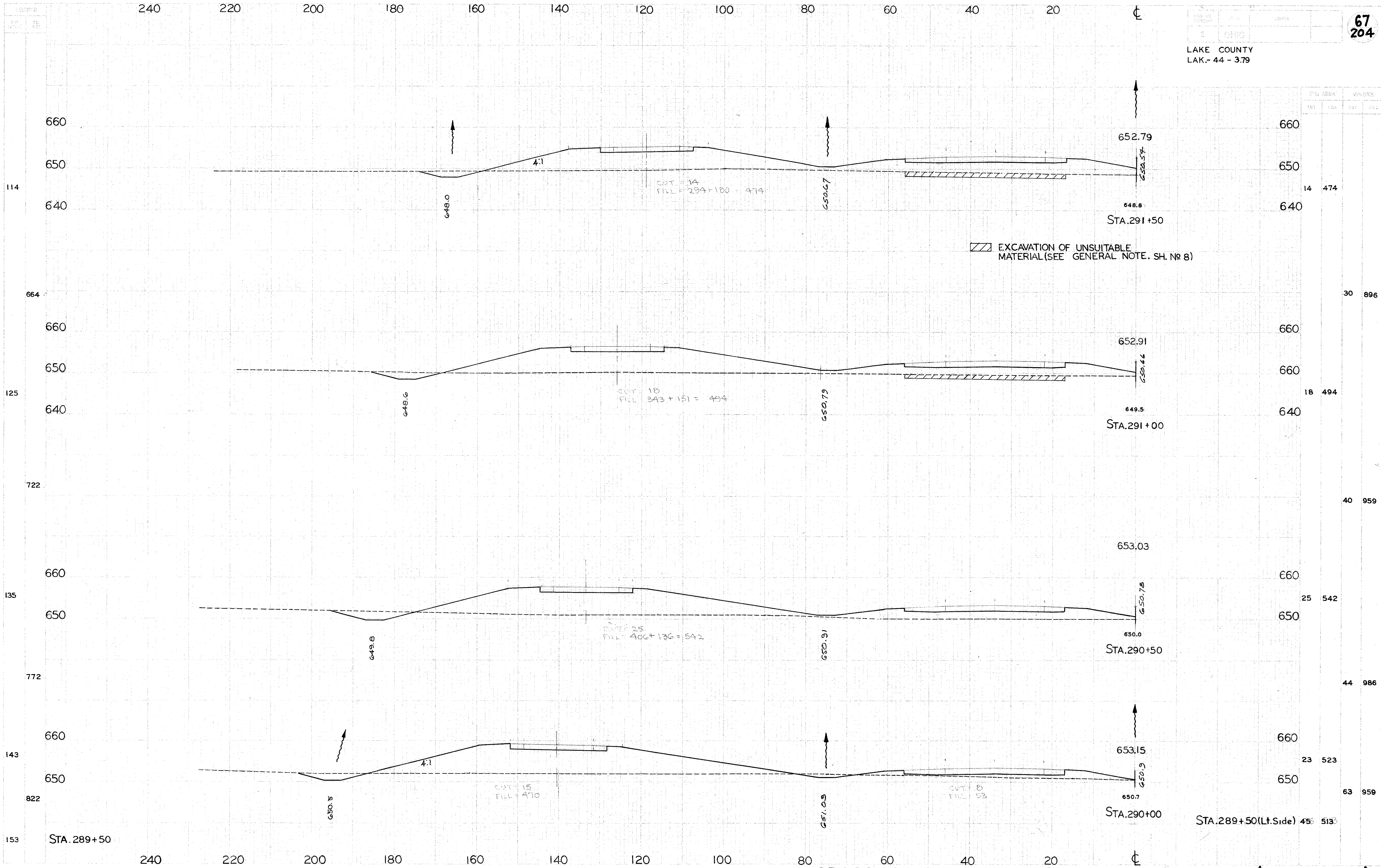
CROSS SECTIONS STA. 290+00 TO STA. 291+50 (LEFT SIDE)
