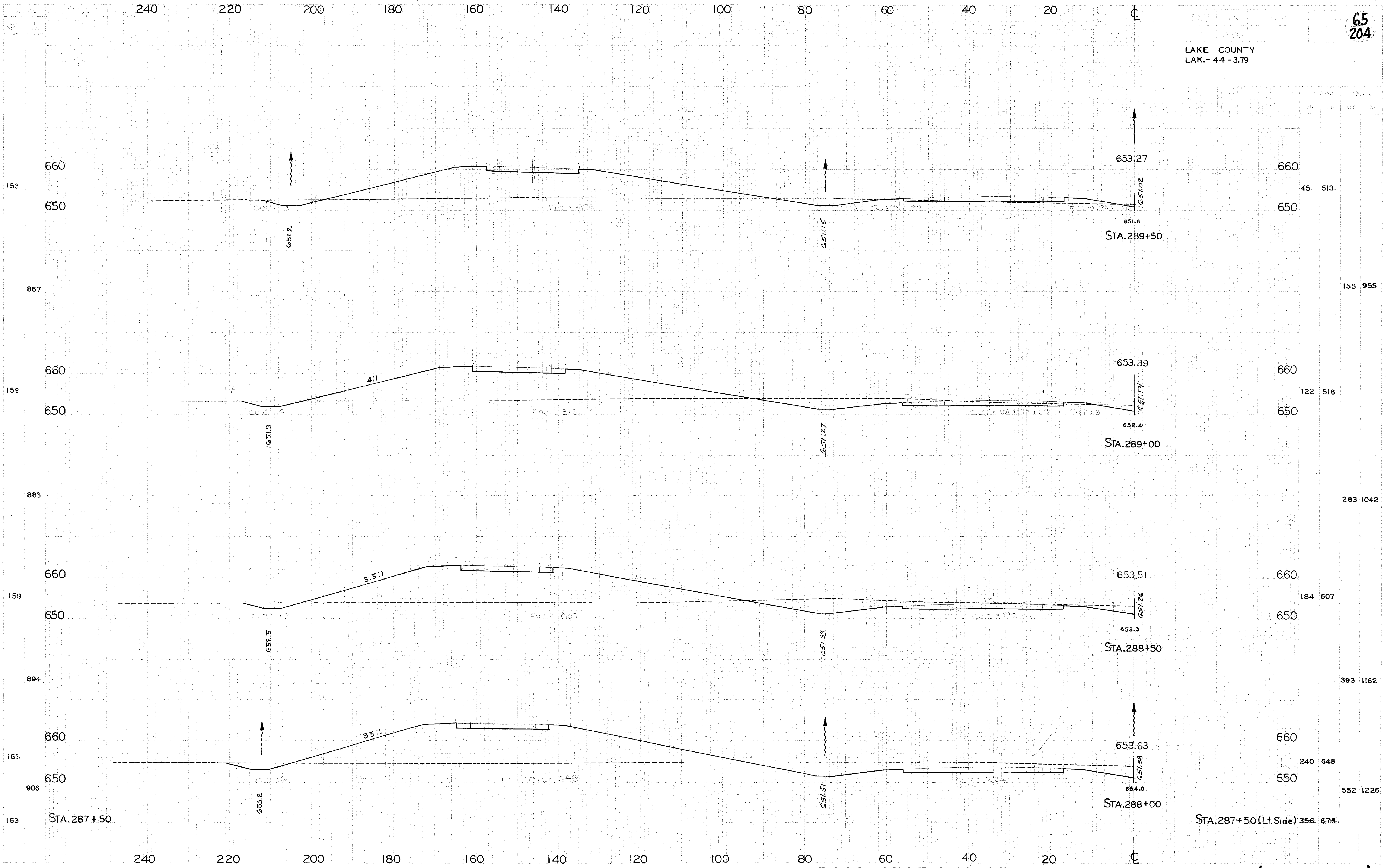
CROSS SECTIONS STA.288+00 TO STA.289+50 (LEFT SIDE)
