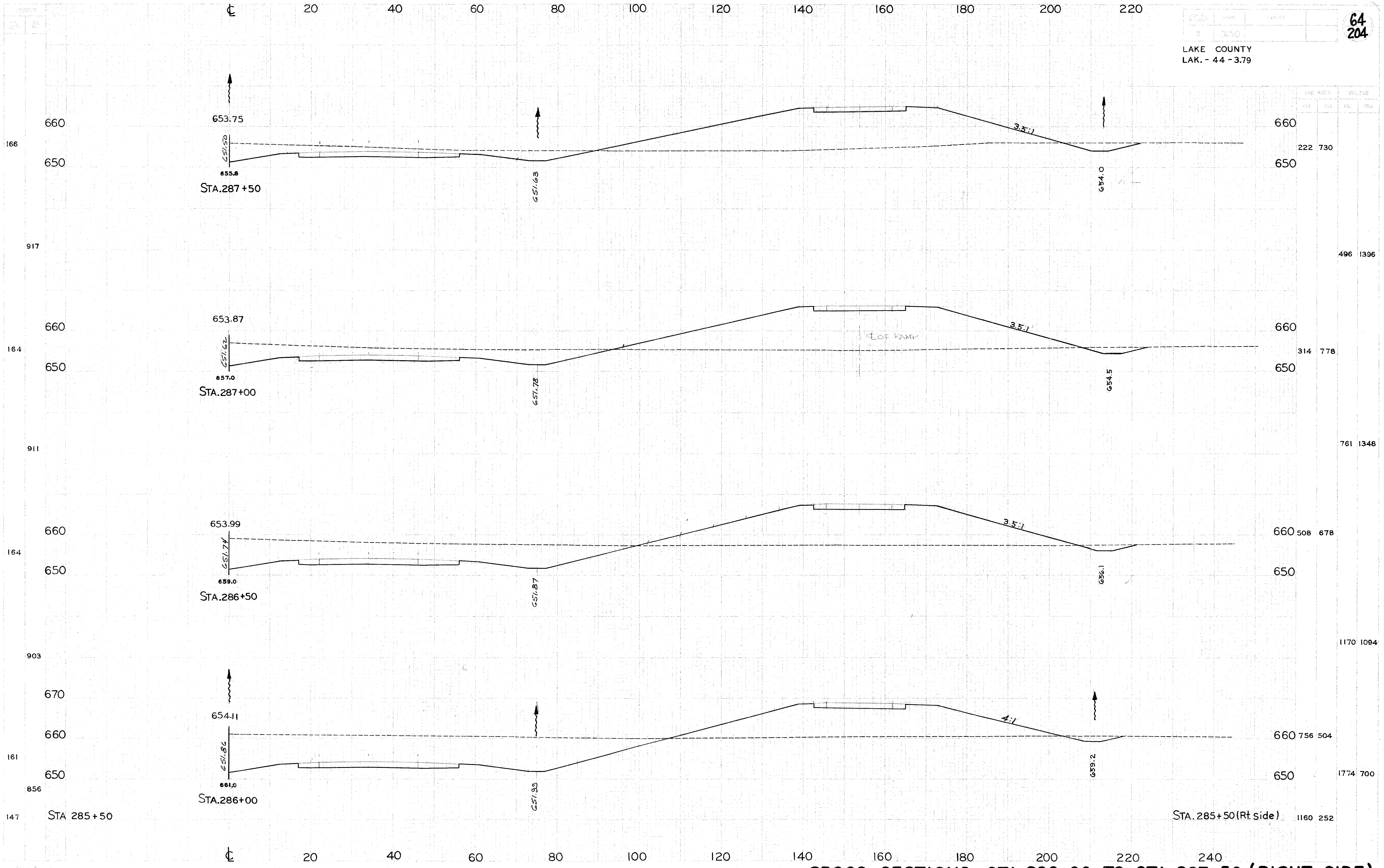
CROSS SECTIONS STA.286+00 TO STA.287+50 (RIGHT SIDE)
