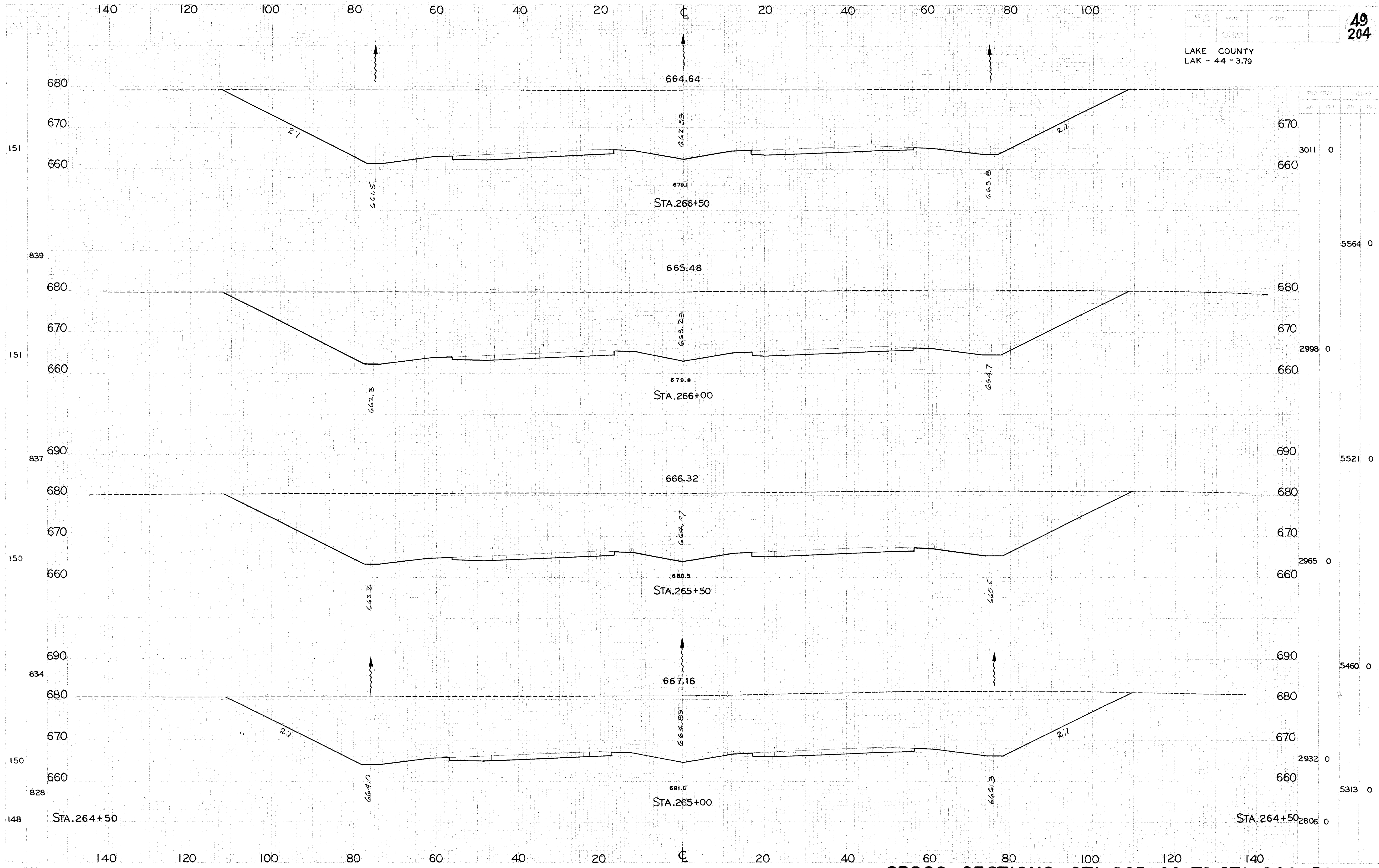
CROSS SECTIONS STA.265+00 TO STA.266+50
