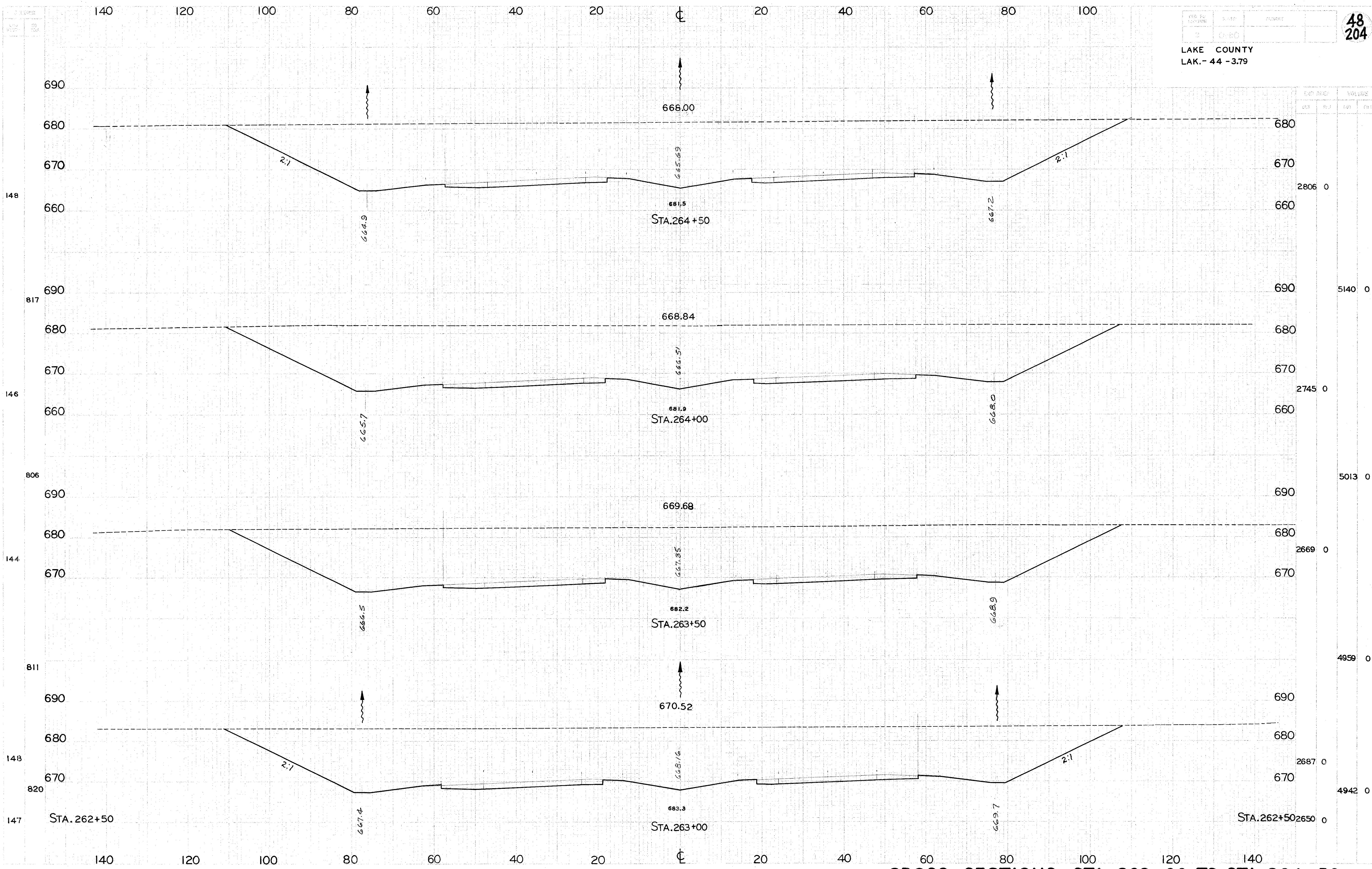
CROSS SECTIONS STA.263+00 TO STA.264+50
