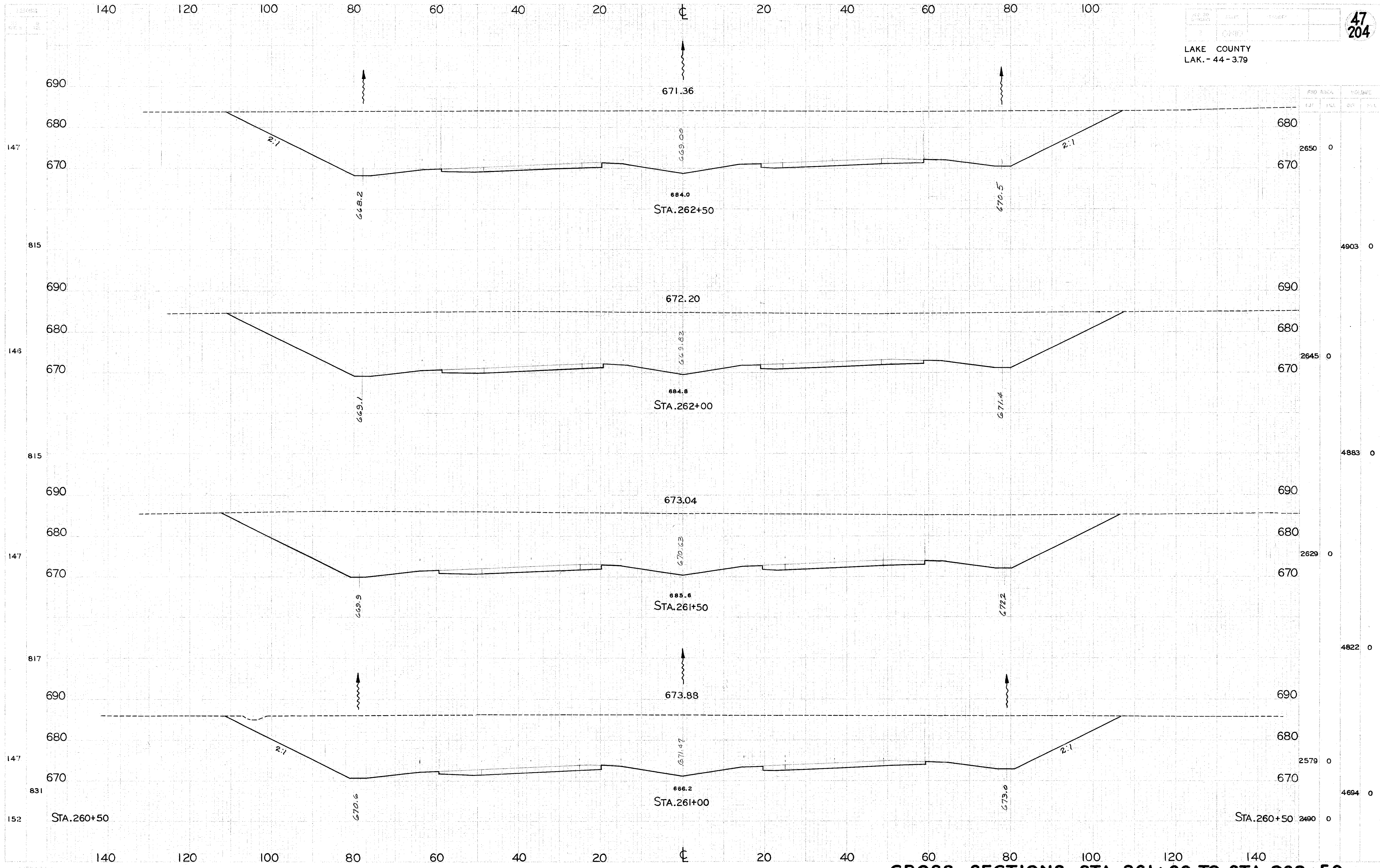
CROSS SECTIONS STA.261+00 TO STA.262+50
