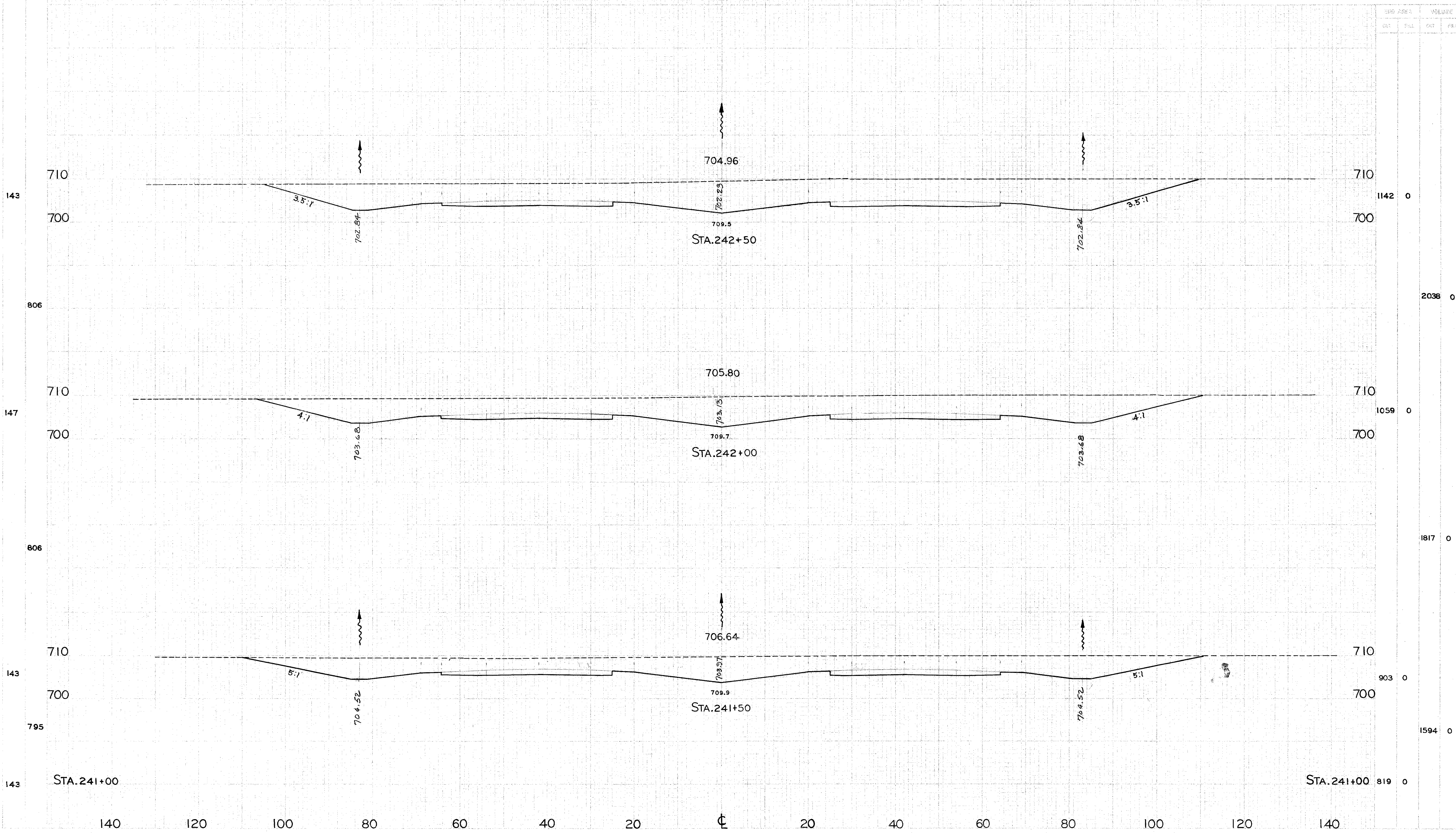
CROSS SECTIONS STA.241+50 TO STA.242+50
