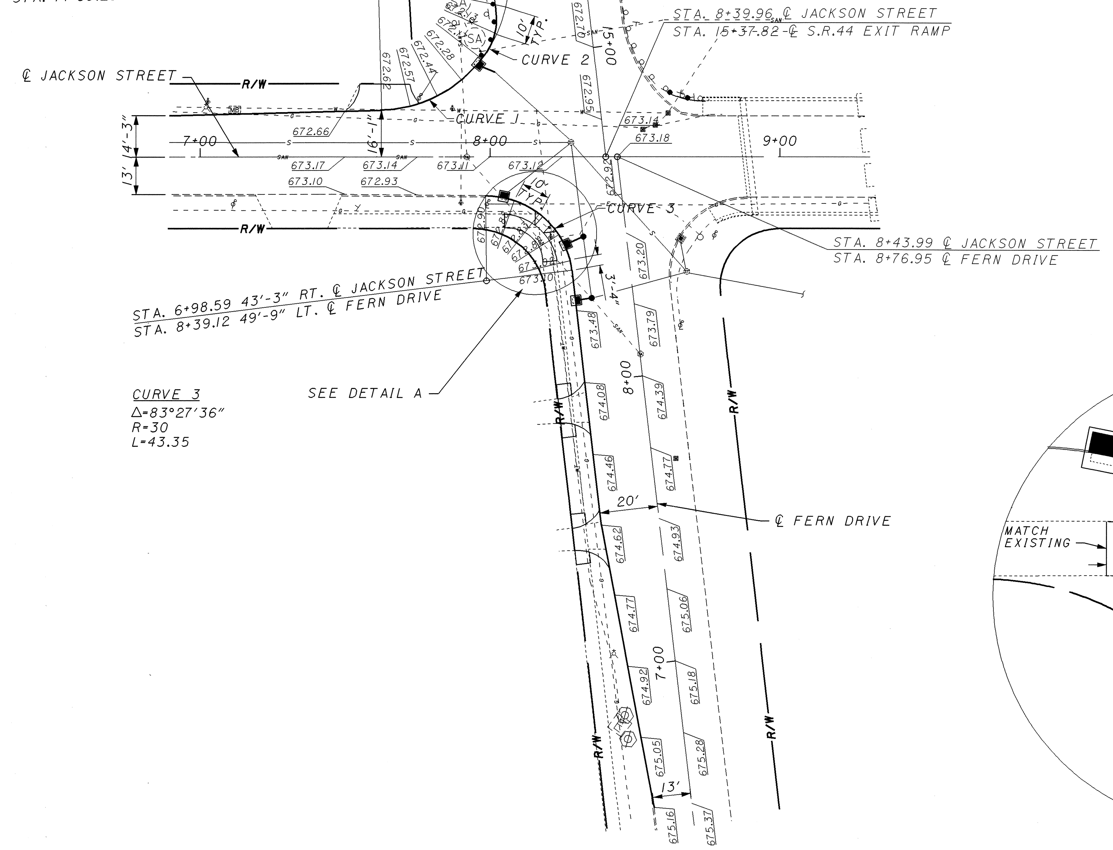
JACKSON STREET - FERN DRIVE - S.R.44 EXIT RAMP INTERSECTION
