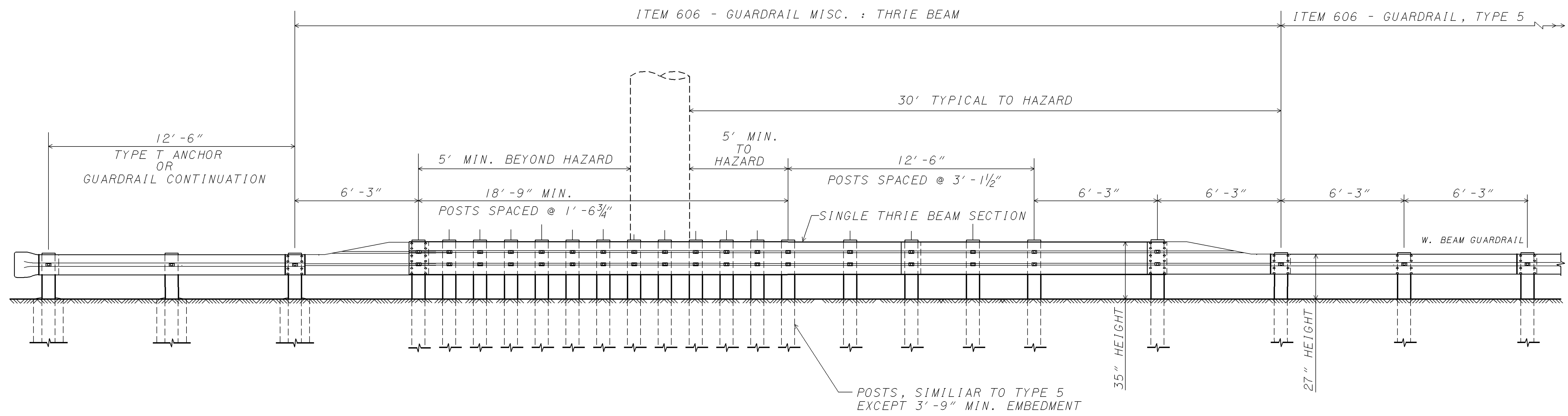
ELEVATION VIEW
