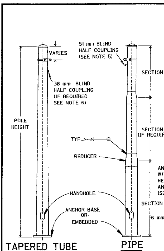
POLE DETAILS
