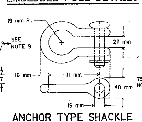
POLE DETAILS
