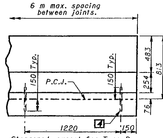
813-mm BARRIER
