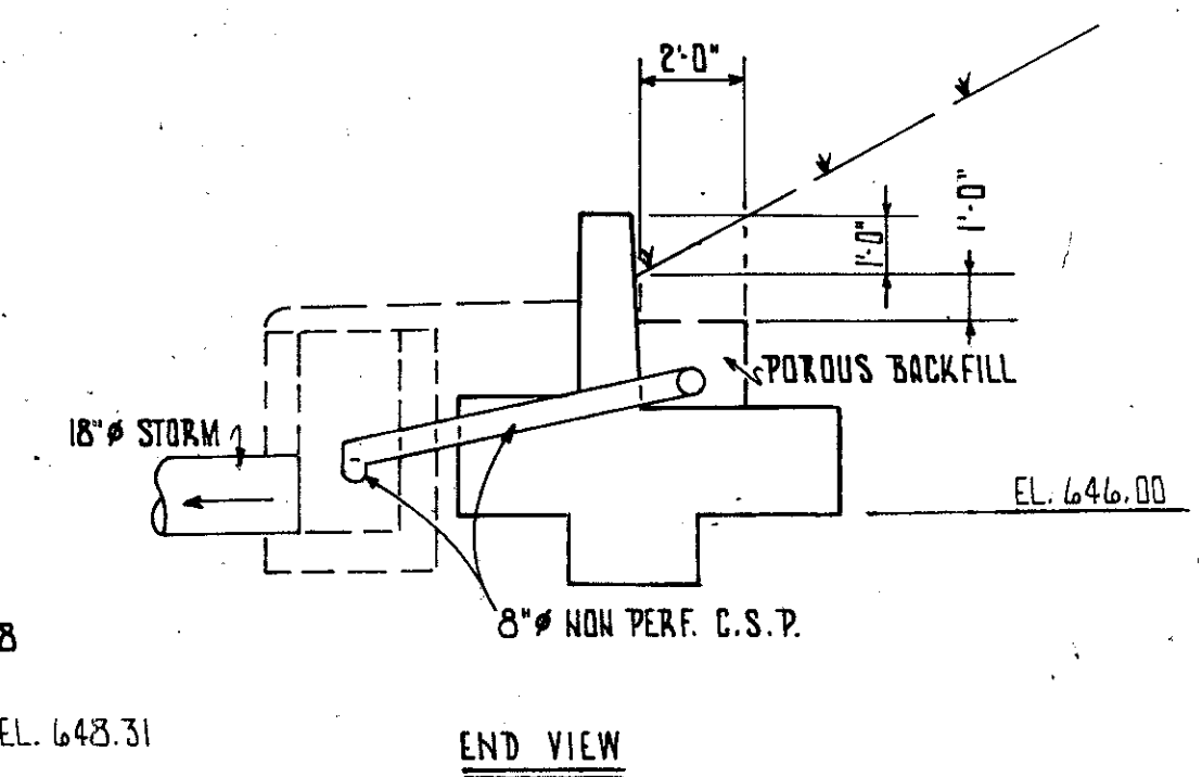
END VIEW
