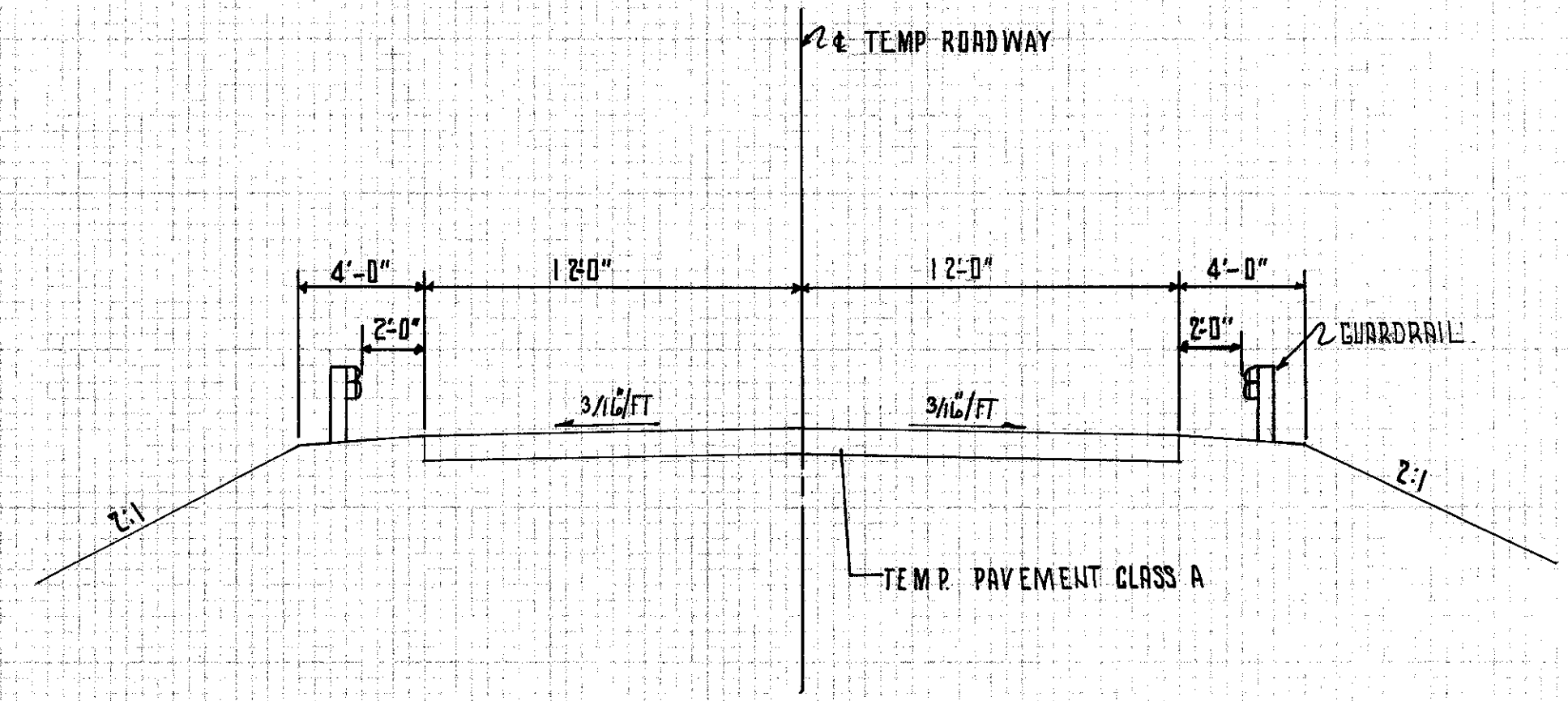
TYPICAL SECTION
