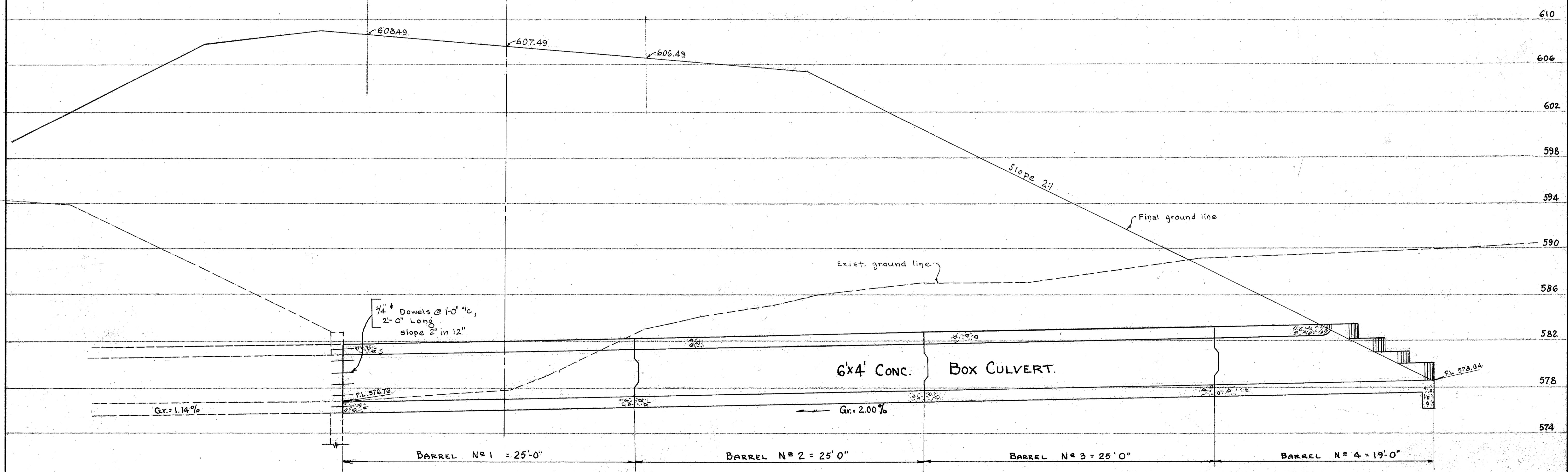
SECTION A-A SCALE 1" = 4'-0" VERT. - 1/4" = 1'-0" HOR.
