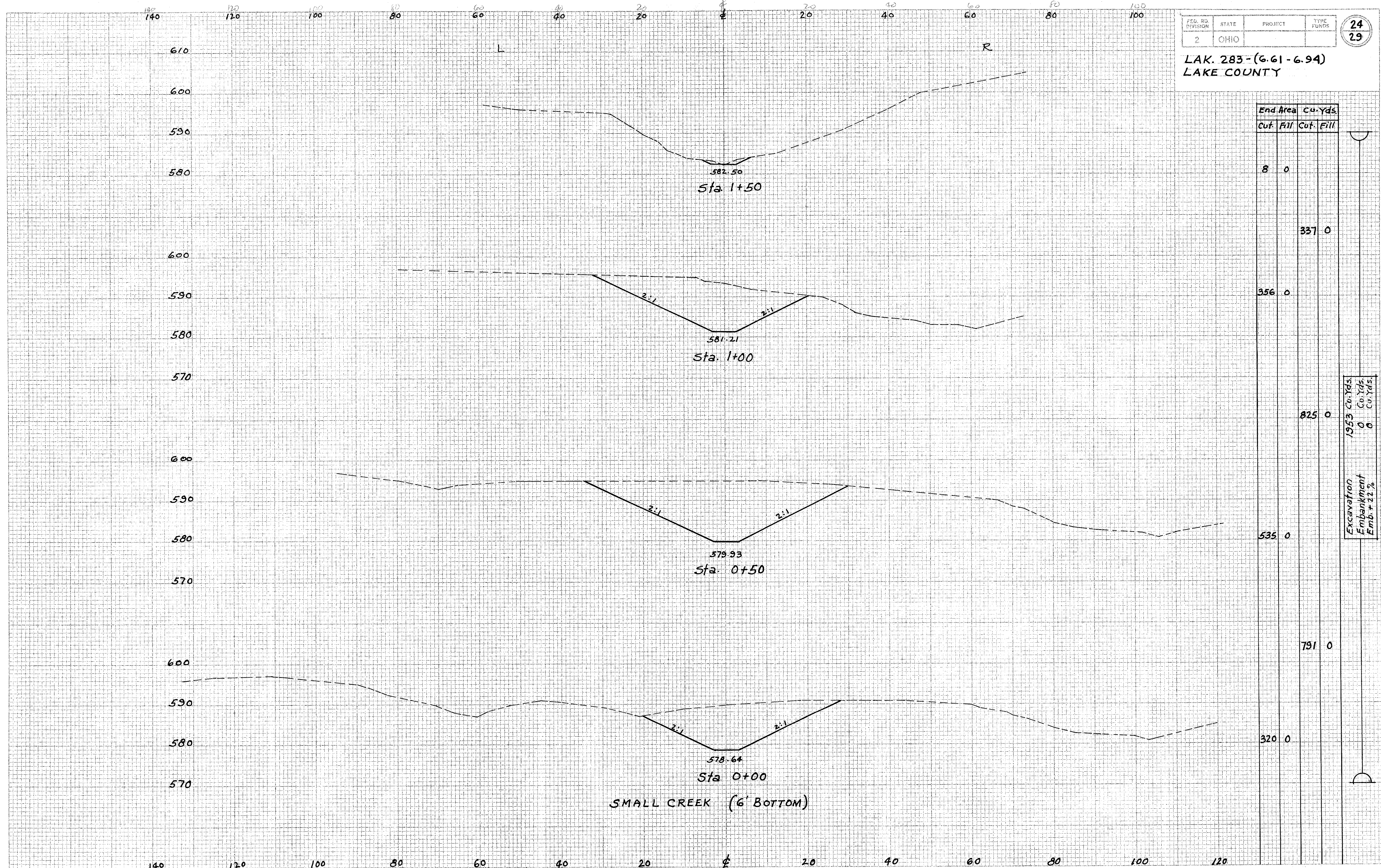
X-SECTIONS - STA. 0+00 TO STA. 1+50 (SMALL CREEK)
