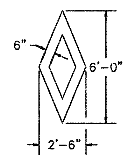
PREFERENTIAL LANE MARKER
