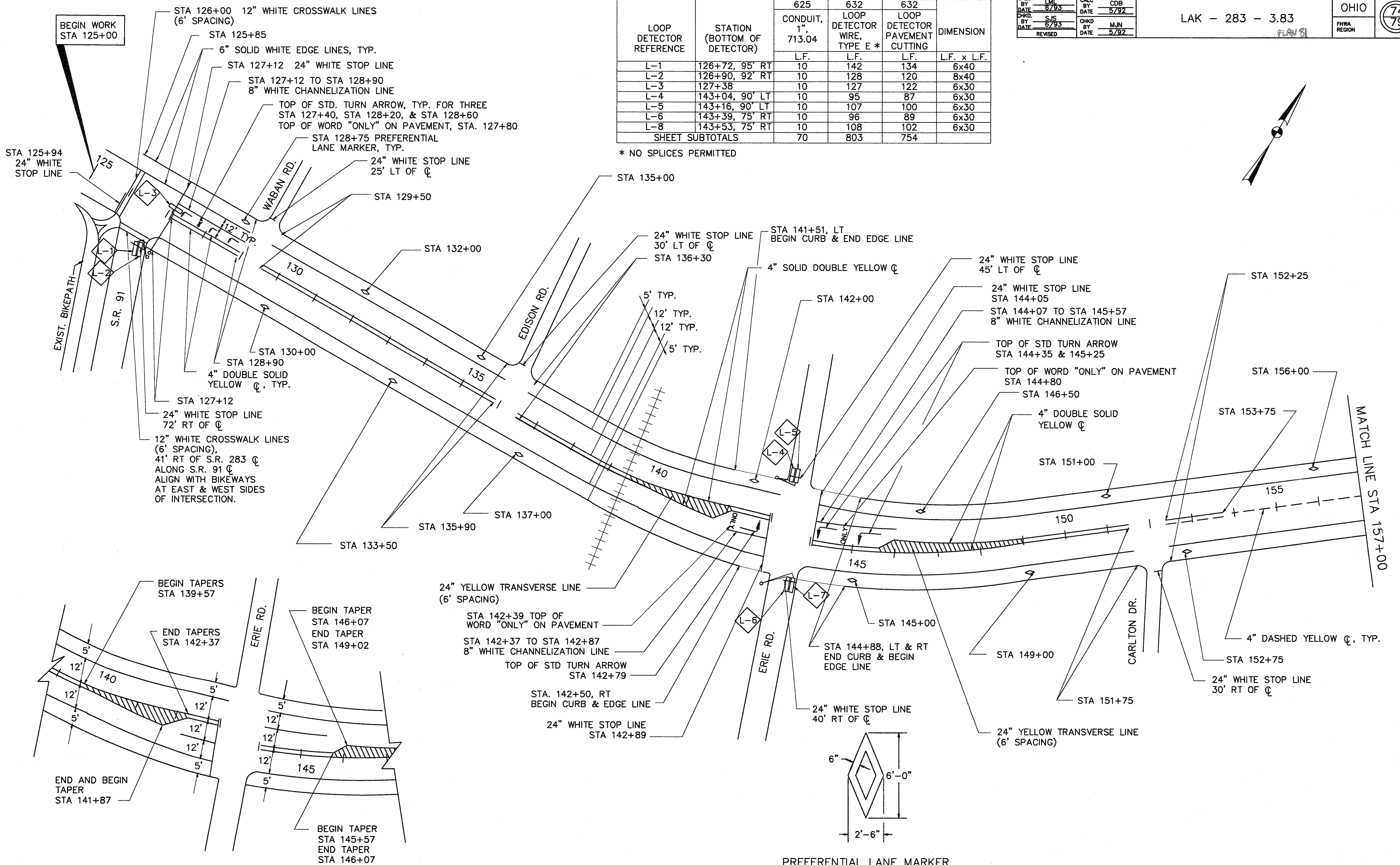
PAVEMENT MARKINGS
