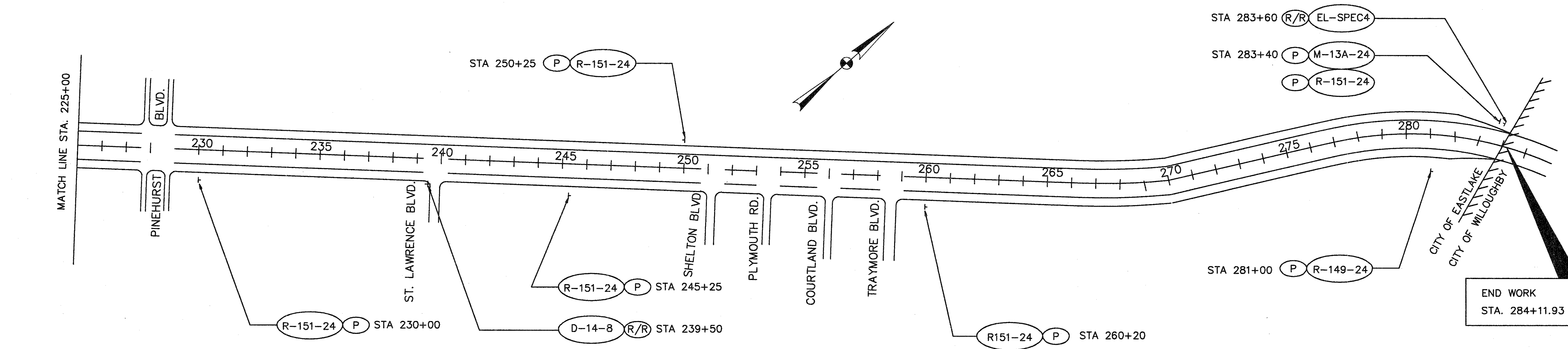
SIGN SCHEMATIC
