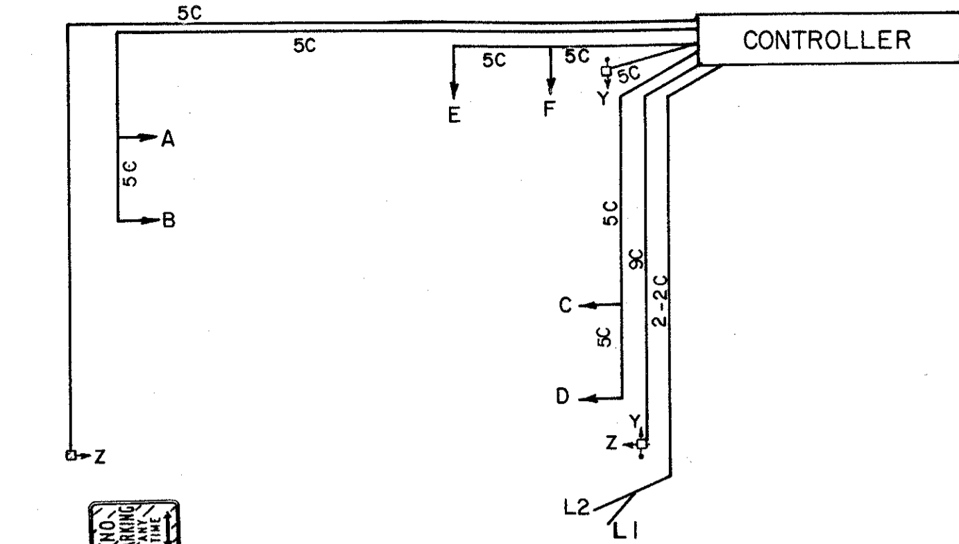
WIRING DIAGRAM
