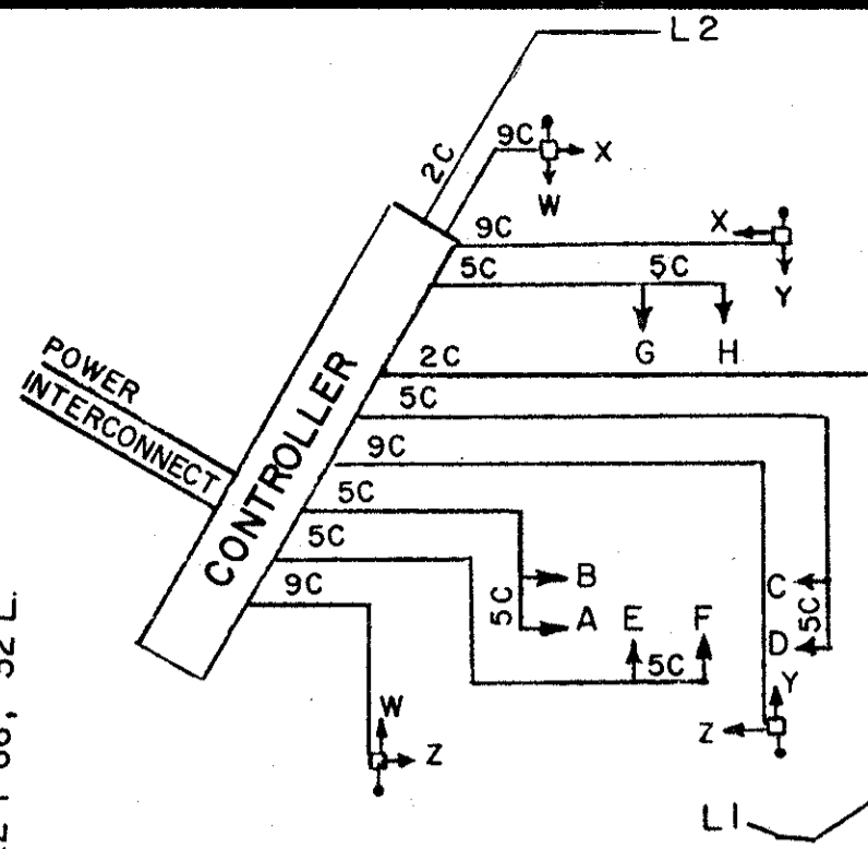
WIRING DIAGRAM
