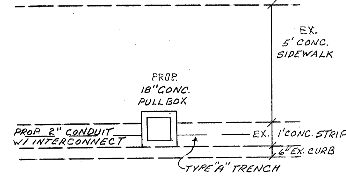
TYPICAL STA. 447+17 TO 471+74
