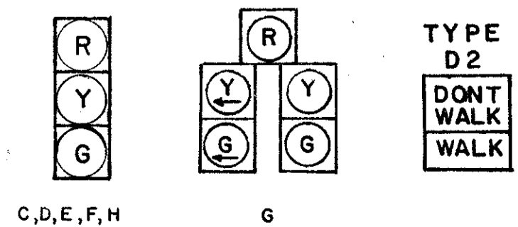
12" SIGNAL HEADS
