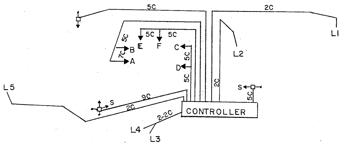
WIRING DIAGRAM
