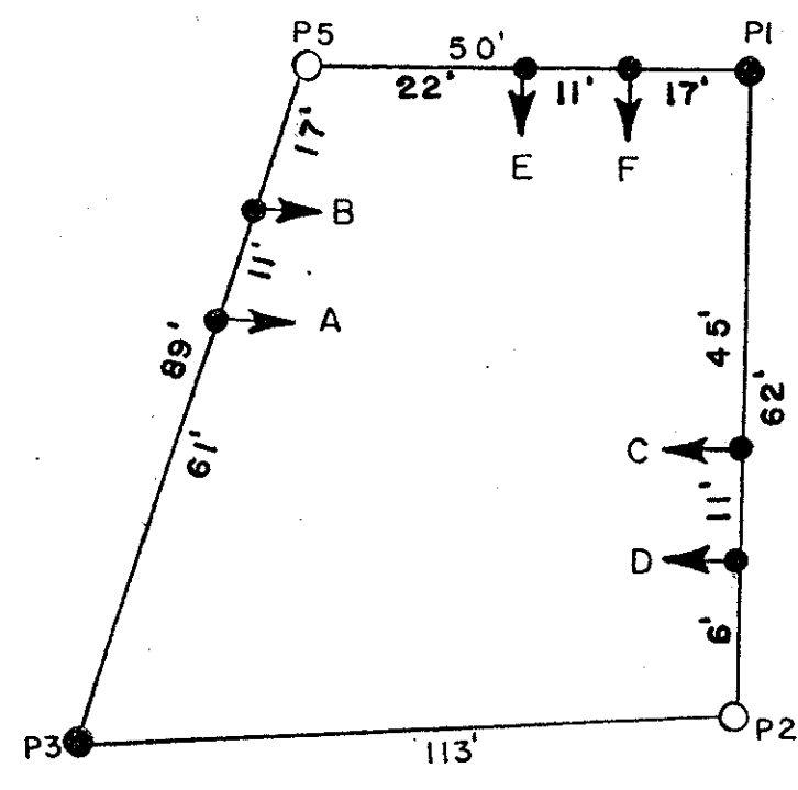
SPAN DIAGRAM
