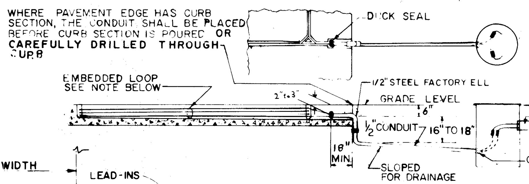
FIGURE 3 TYPICAL TWO LANE LOOP INSTALLATION
