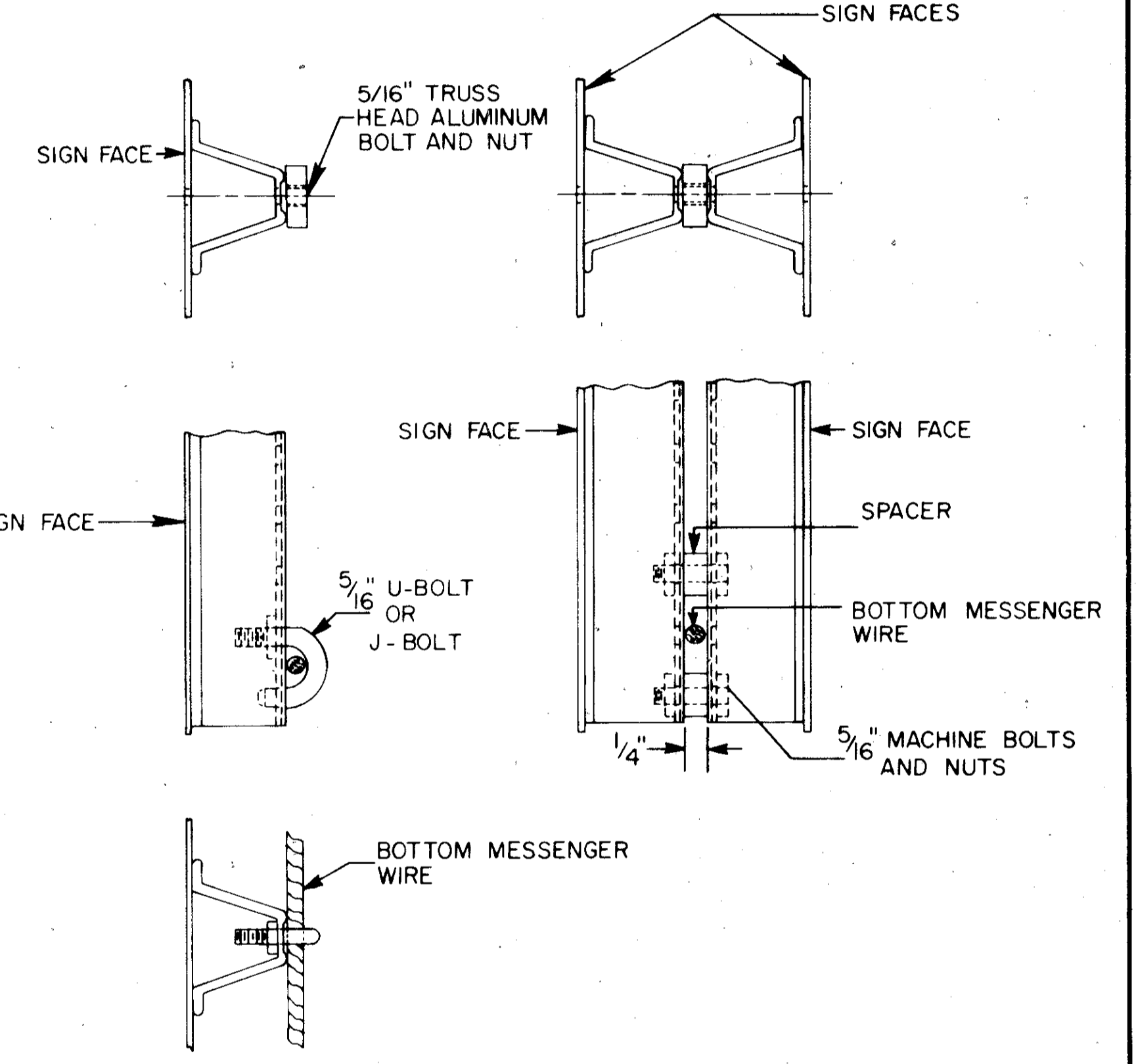
SIGN ATTACHMENT DETAILS
