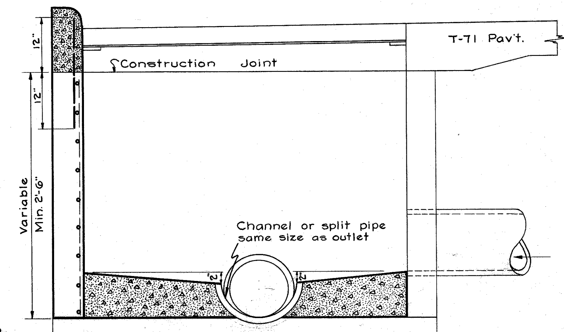
SECTION B-B
