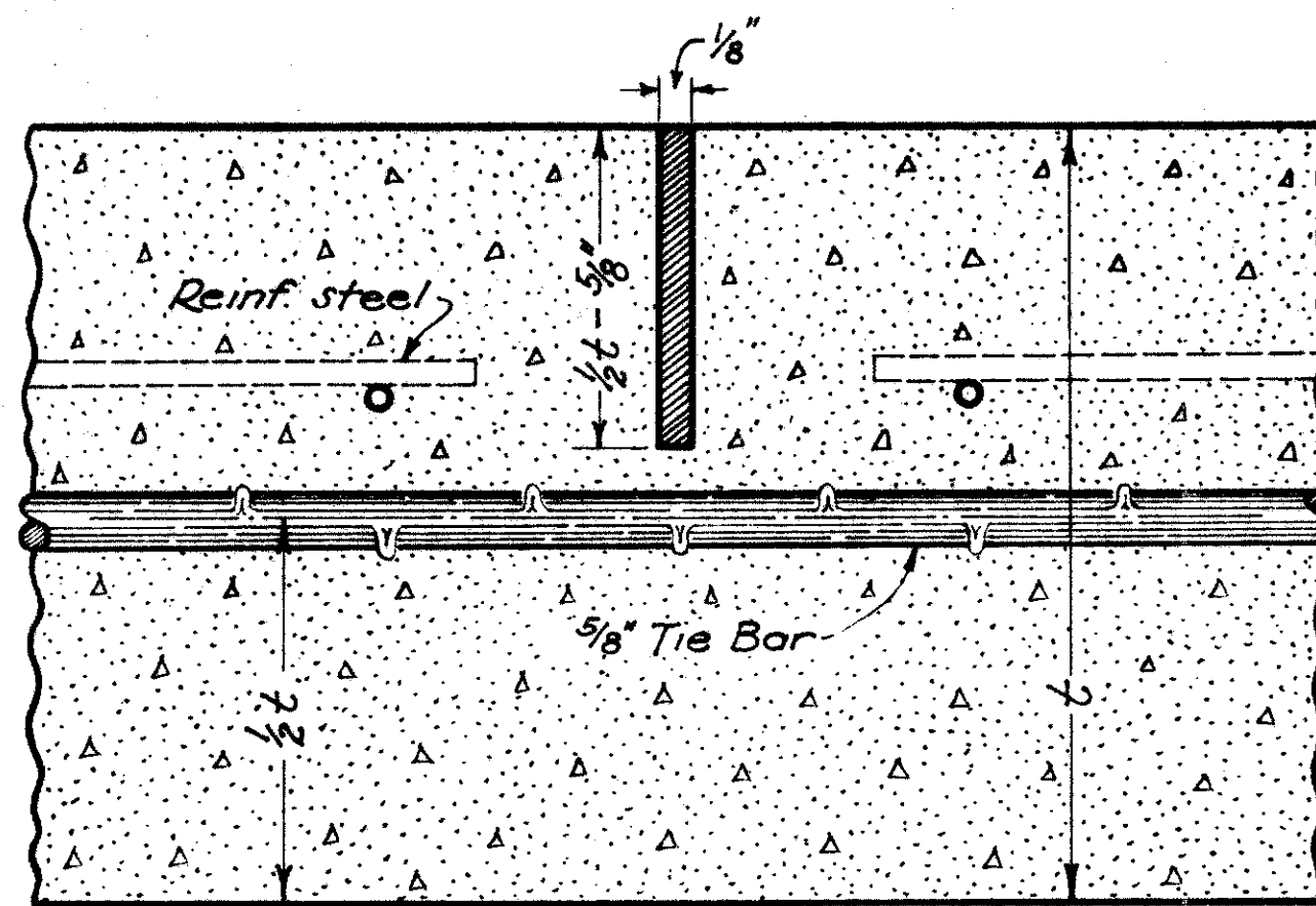
PREMOLDED JOINT
