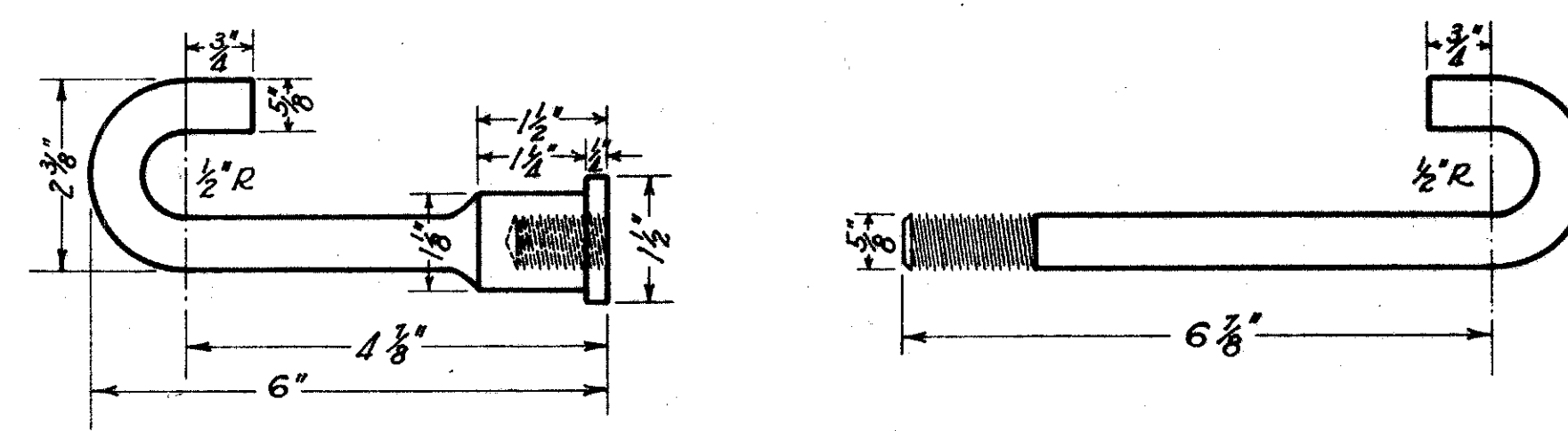
INSERT J BOLT HOOK BOLT DETAIL
