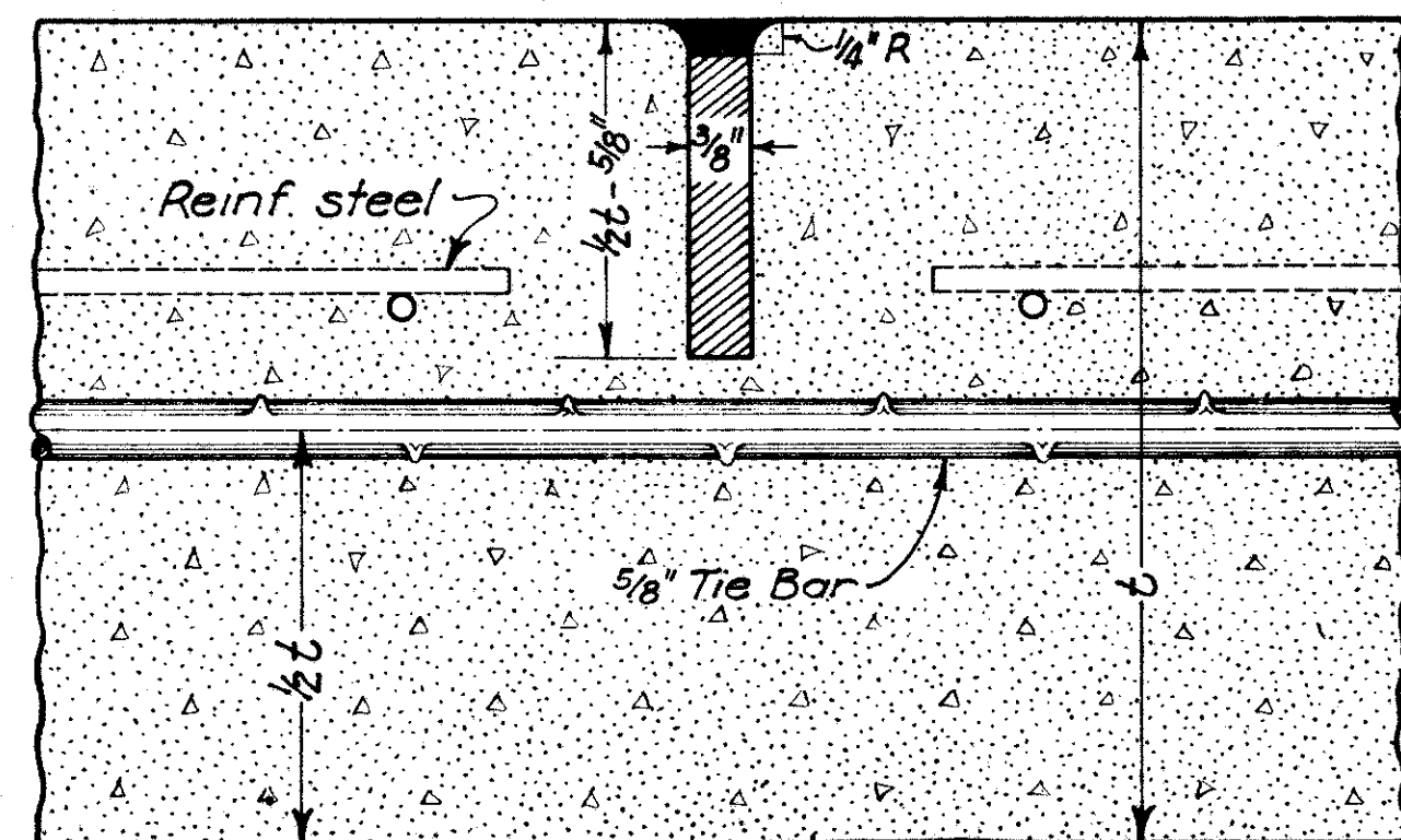
PREMOLDED JOINT
