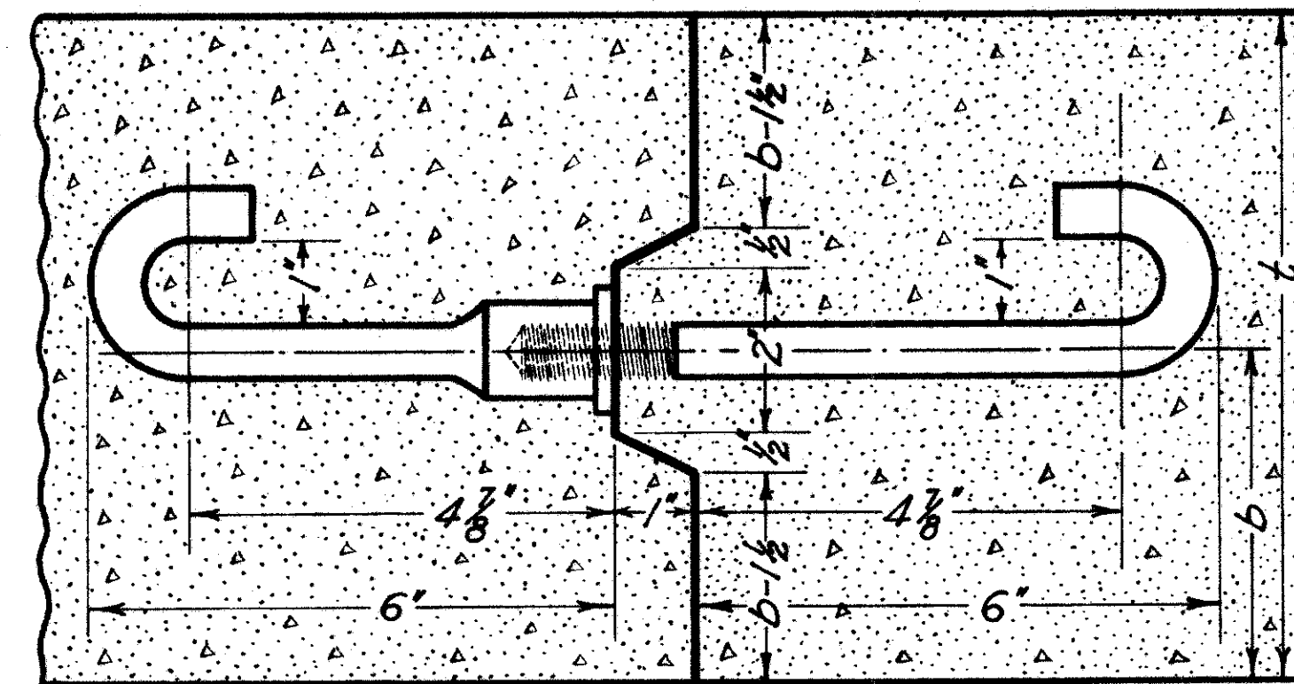
HOOK BOLT AND KEY JOINT
