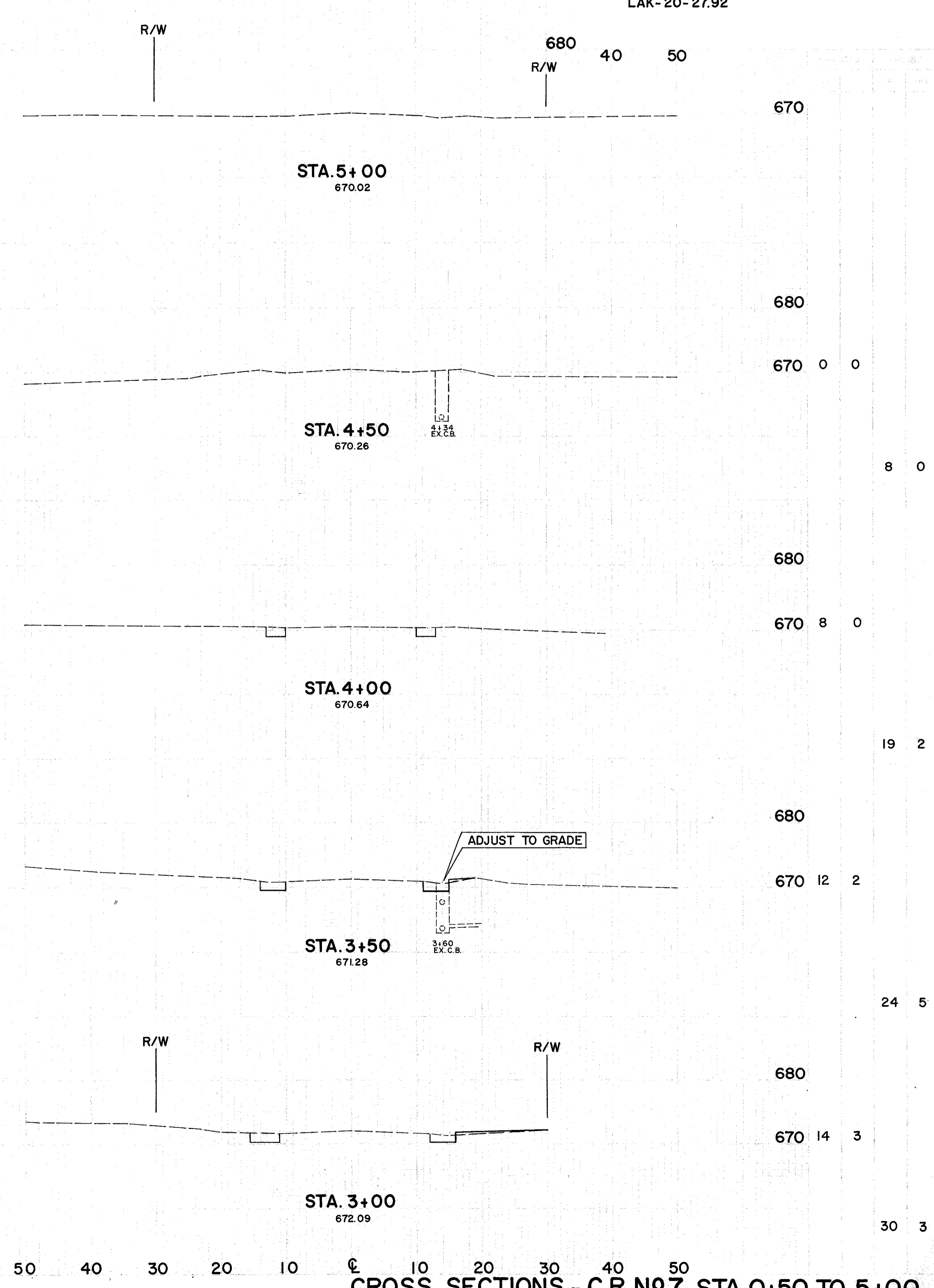
CROSS SECTIONS - C.R. NO 7 - STA. 0+50 TO 5+00
