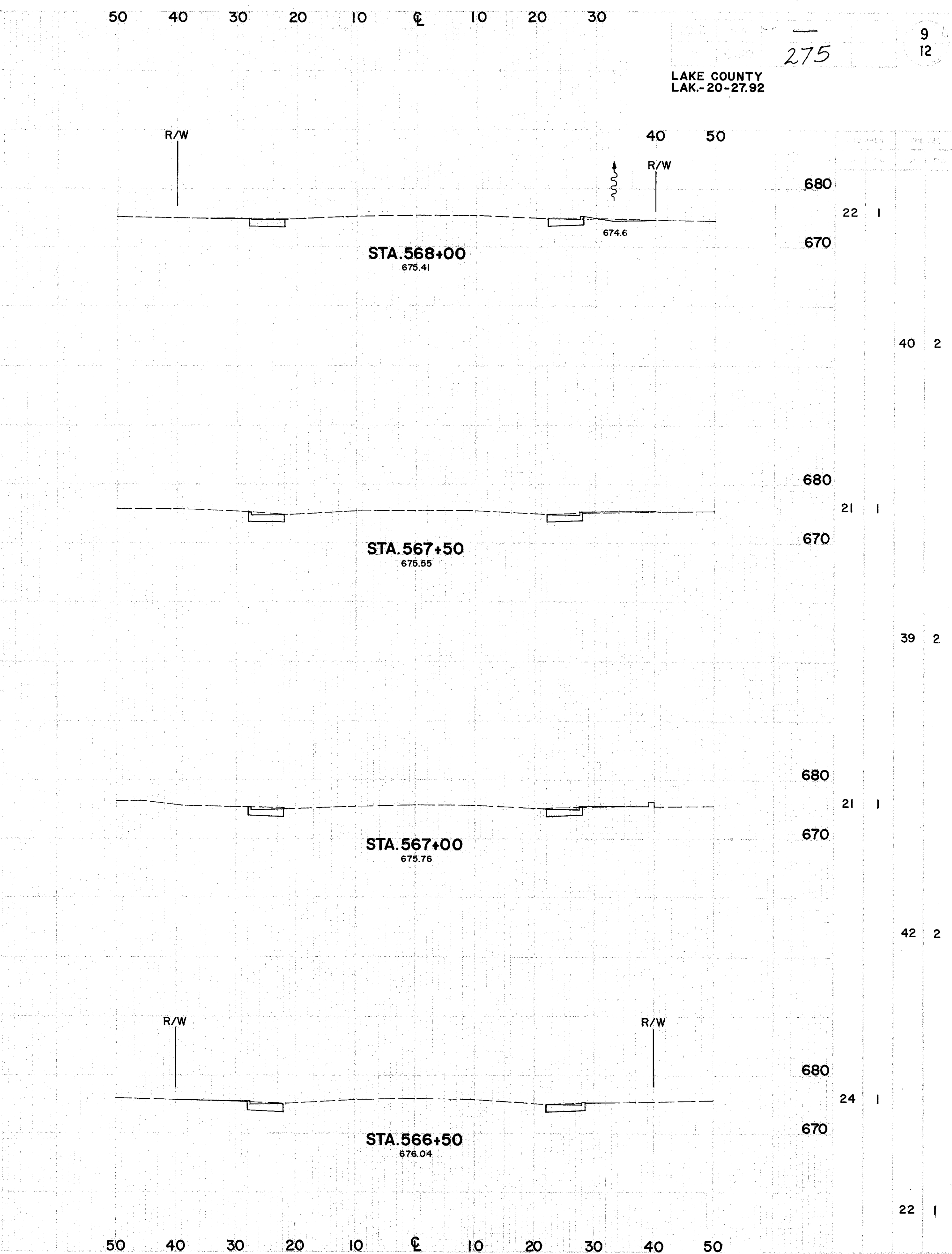
CROSS SECTIONS-S.R.20- STA.564+50 TO 568+00
