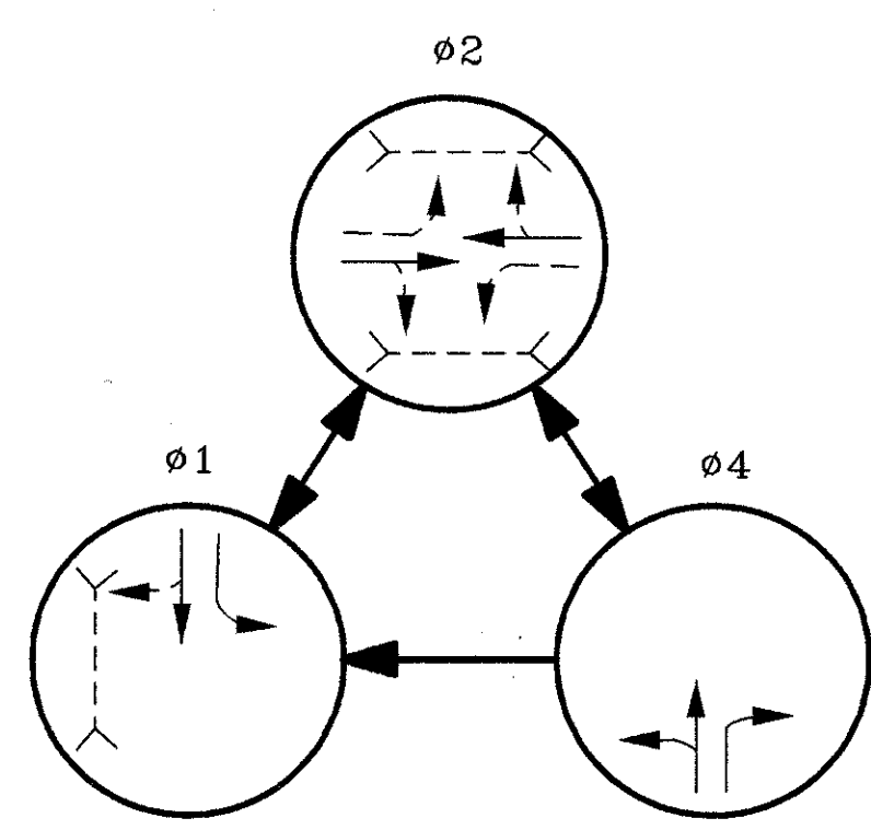
PHASING DIAGRAM
