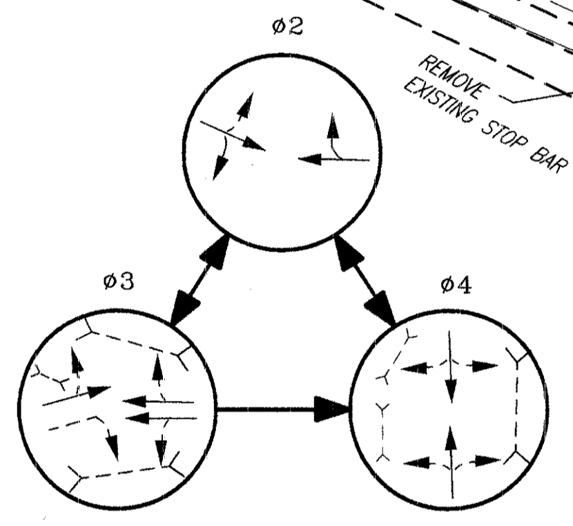
PHASING DIAGRAM
