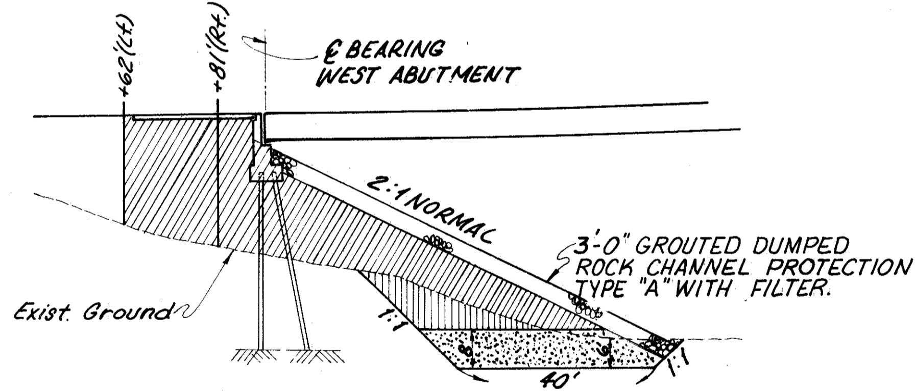
DETAIL FOR FILL PLACEMENT AT WEST BRIDGE ABUTMENT
