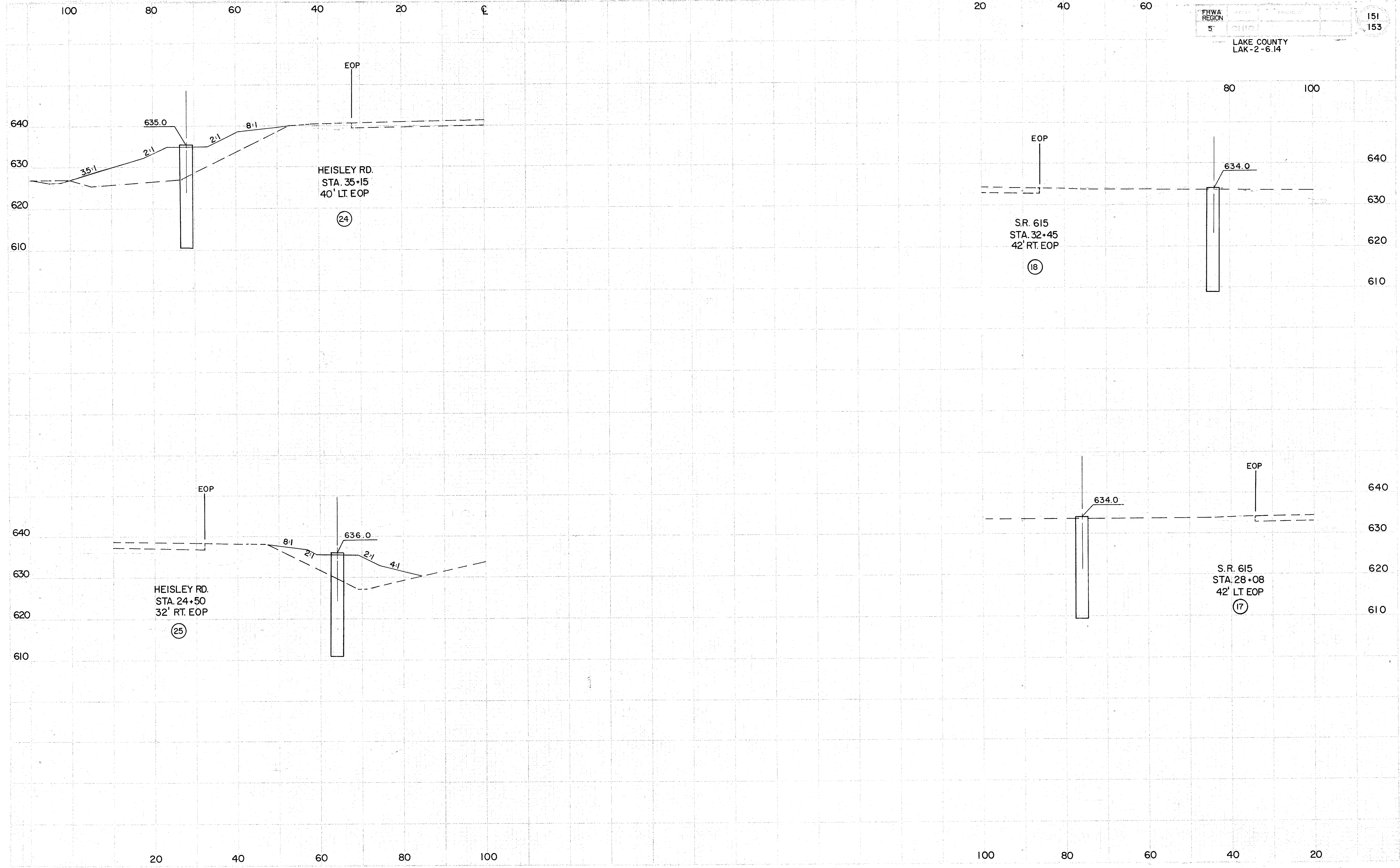
TOWER FOUNDATION CROSS SECTIONS
