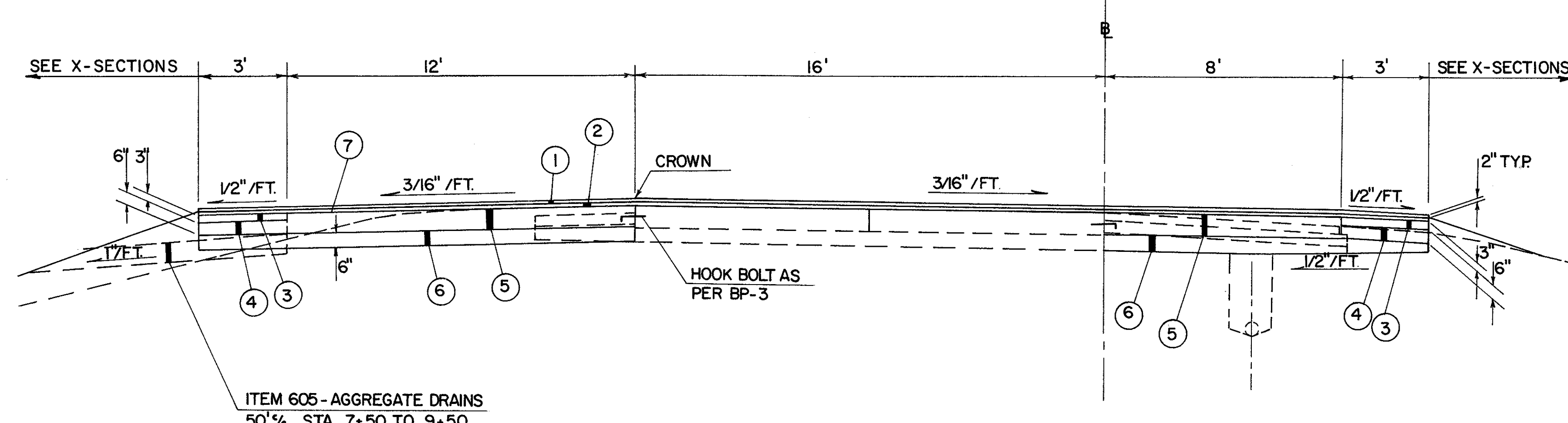
TYPICAL SECTION RAMP G-4 STA. 6+56.84 TO STA. 11+83.27
