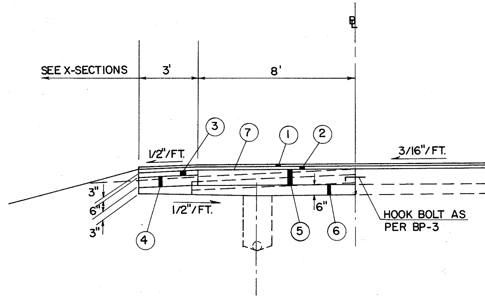
TYPICAL SECTION RAMP G-2 STA. 3+72.71 TO STA. 10+00
