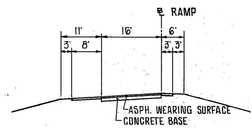
EXISTING RAMP TYPICAL
