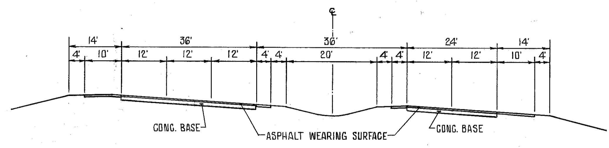
TYPICAL SECTION ~ EXISTING S.R. 2
