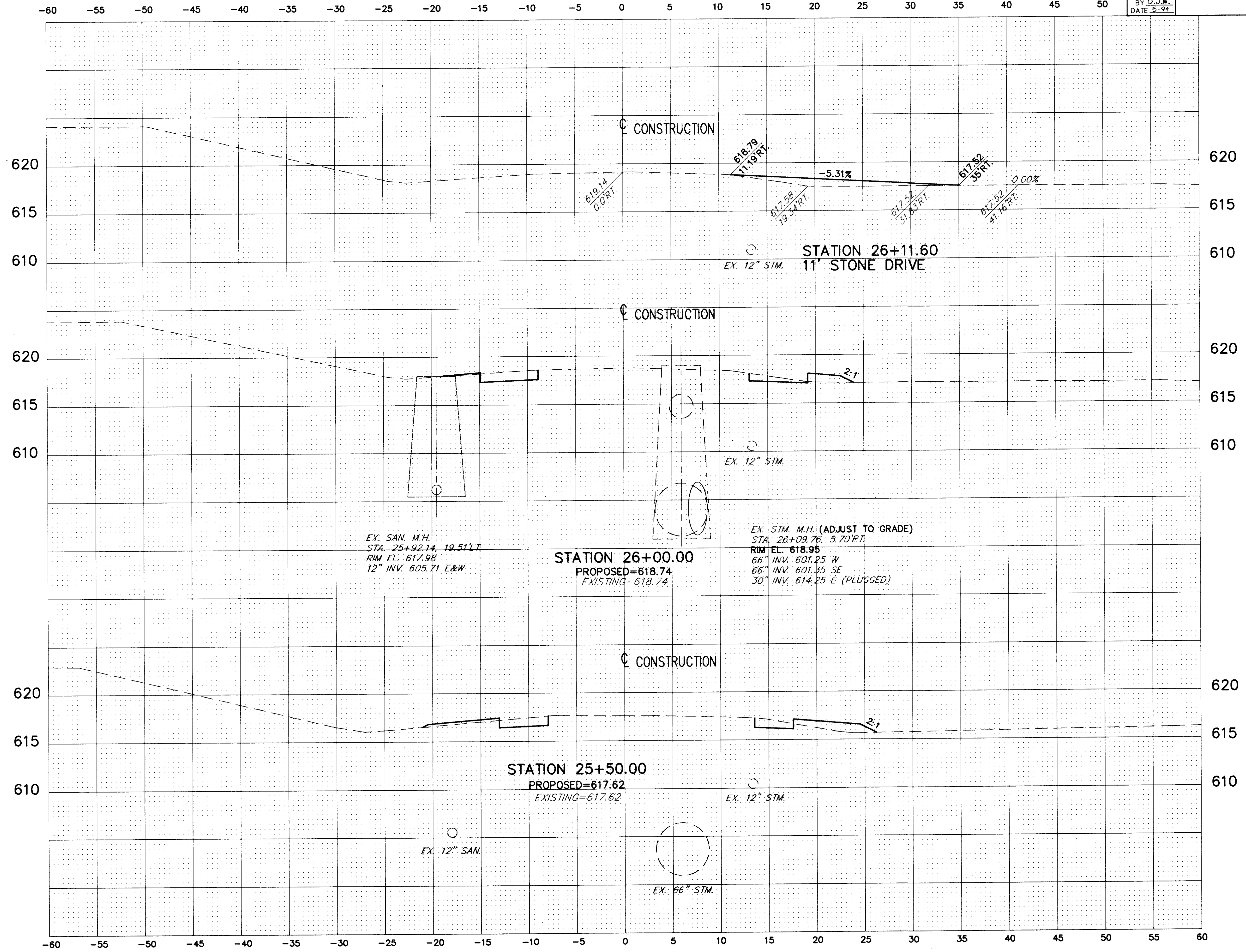
CROSS SECTION STA.25+50 TO STA.26+11.60
