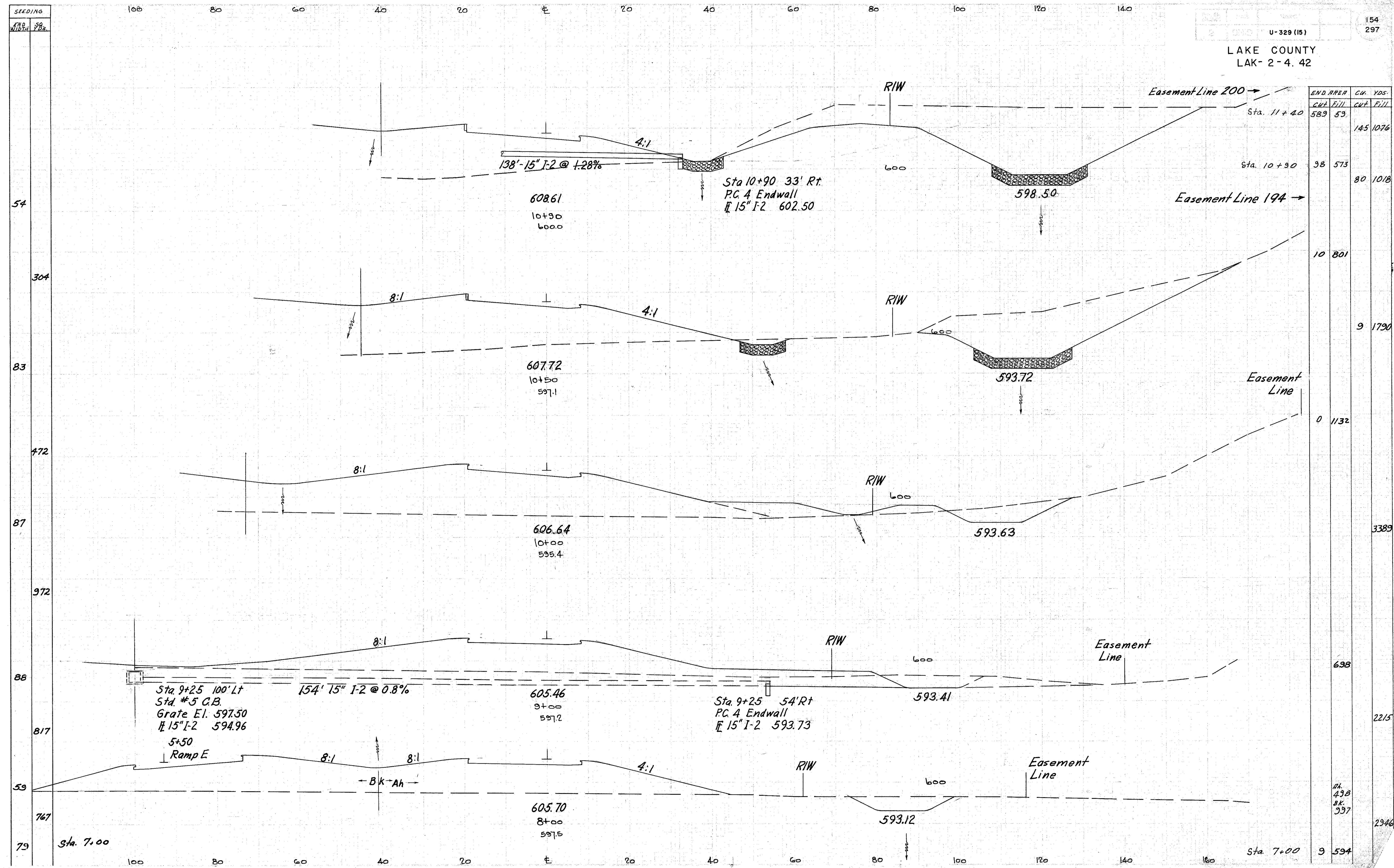
LOST NATIONS ROAD INTERCHANGE RAMP F Sta 8+00 to Sta 10+90
