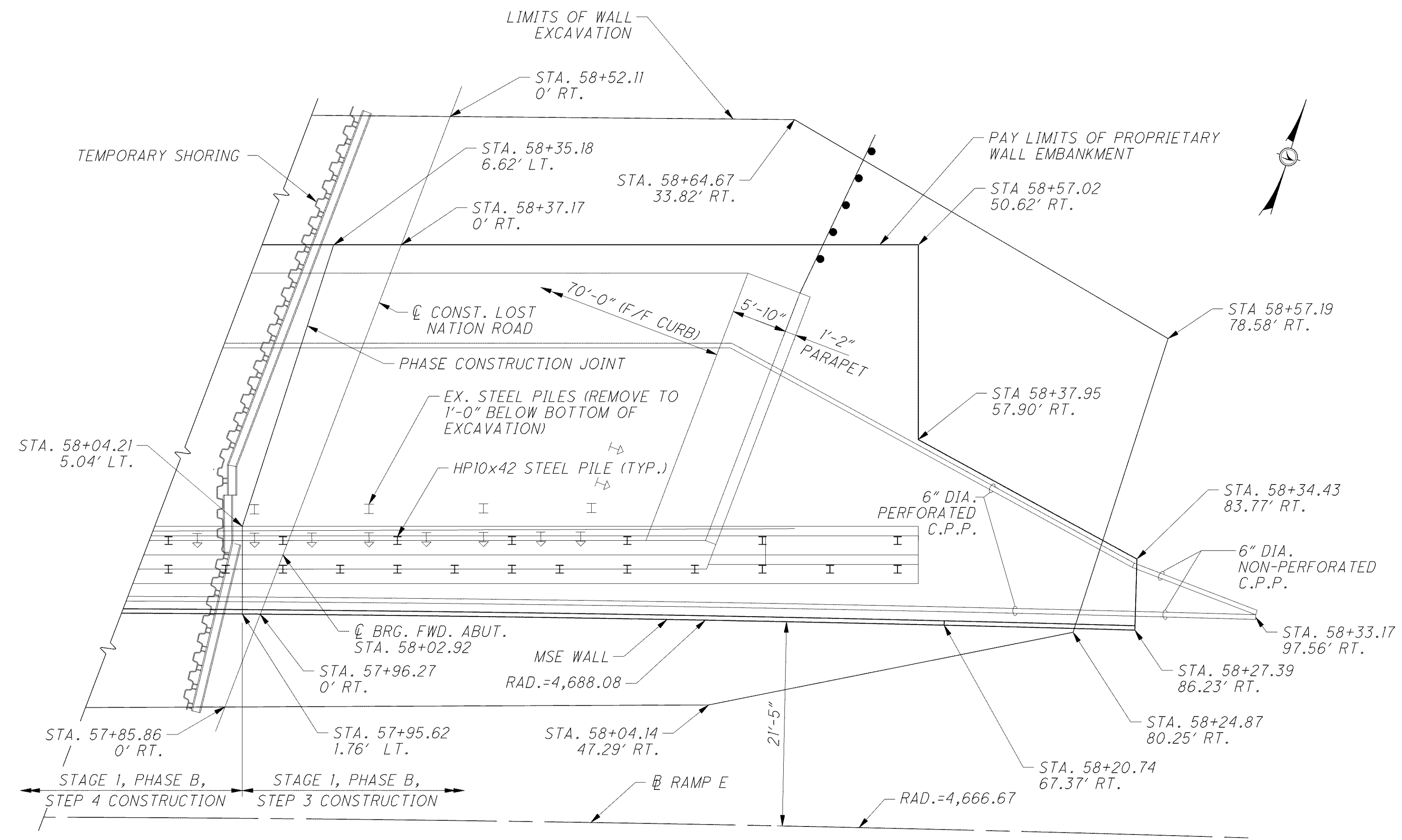
PLAN
