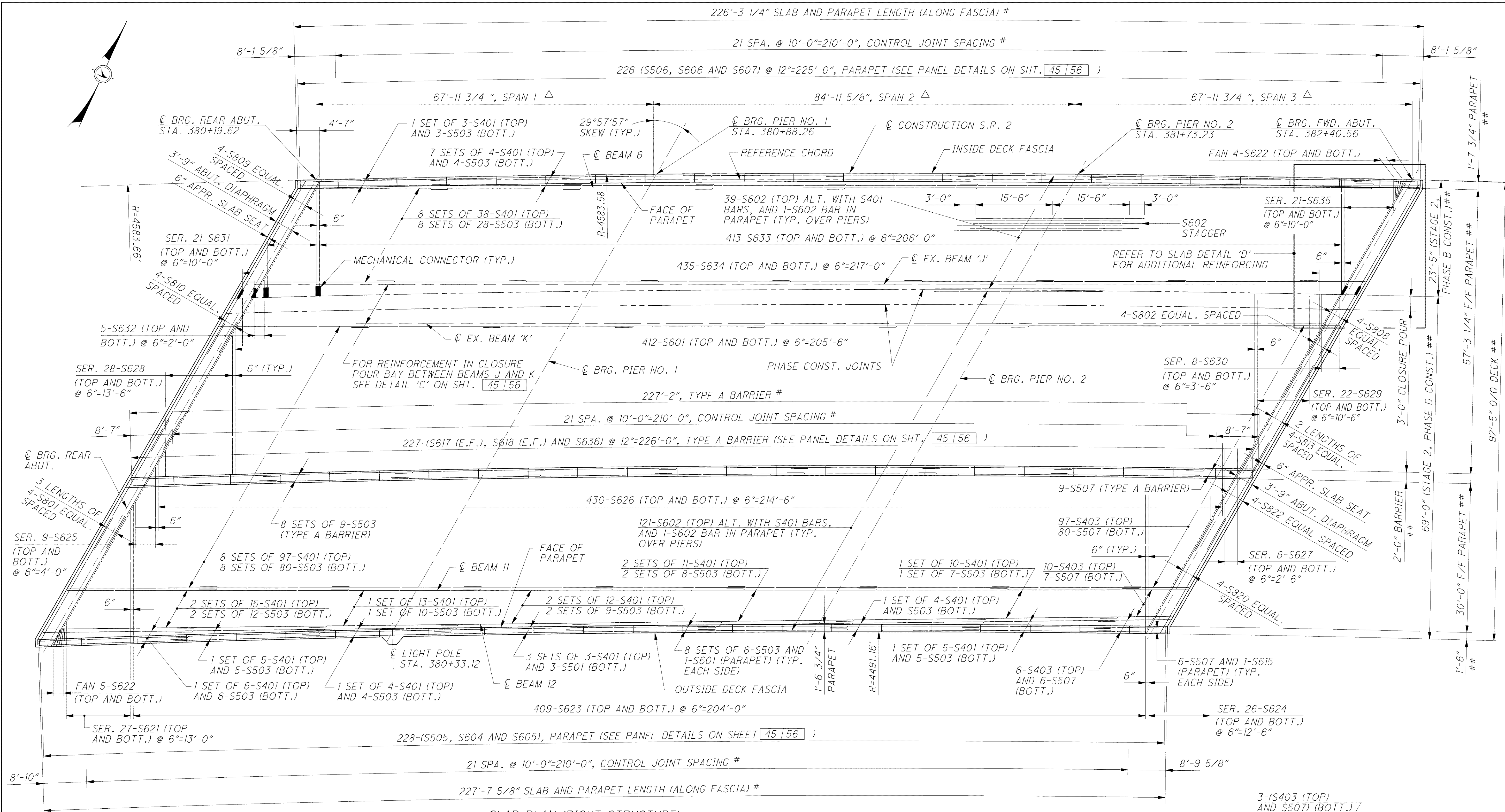
SLAB PLAN (RIGHT STRUCTURE)
