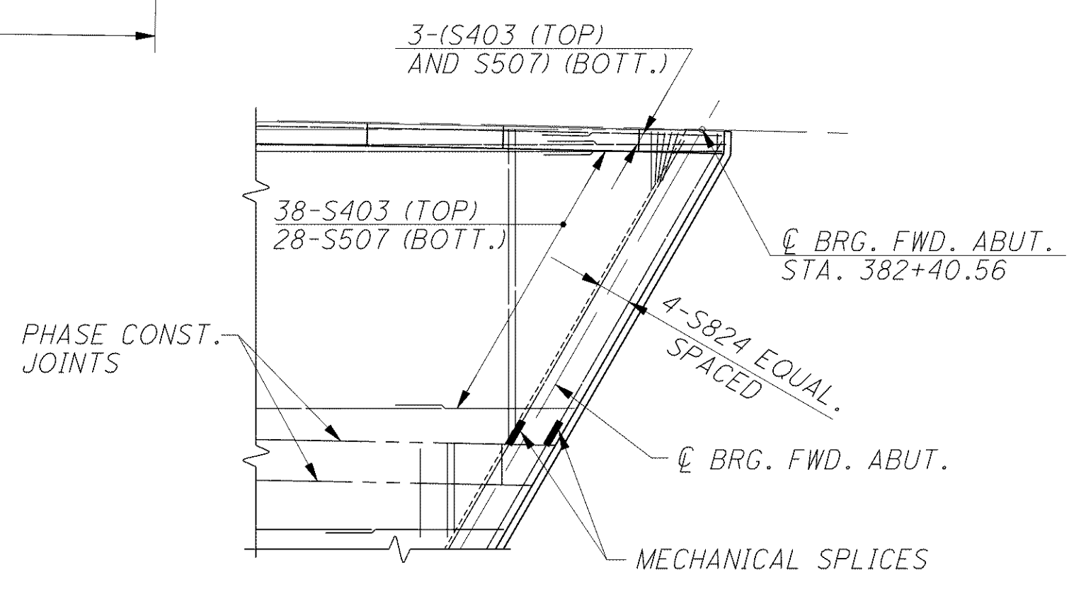
SLAB DETAIL 'D'
