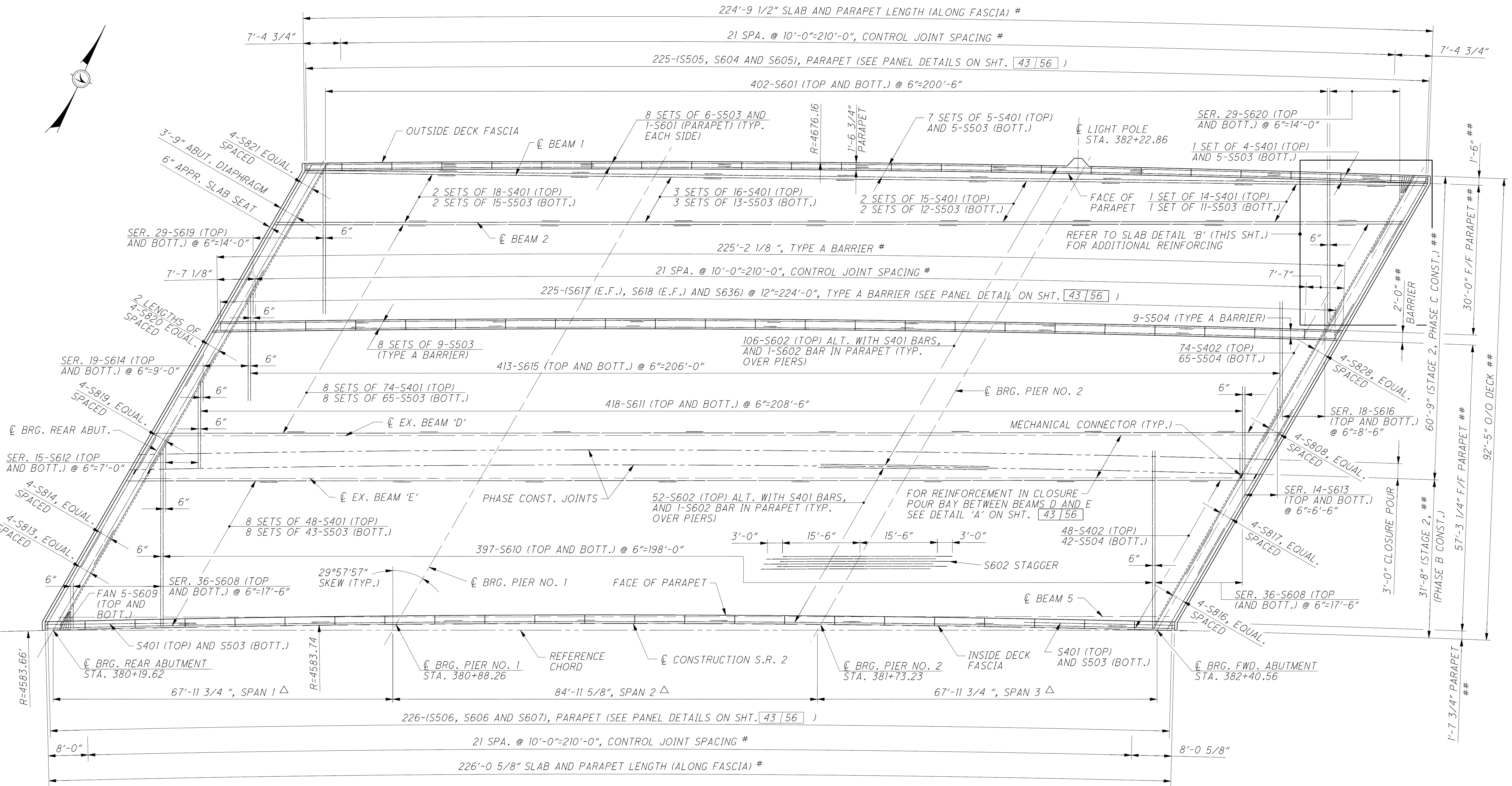
SLAB PLAN (LEFT STRUCTURE)
