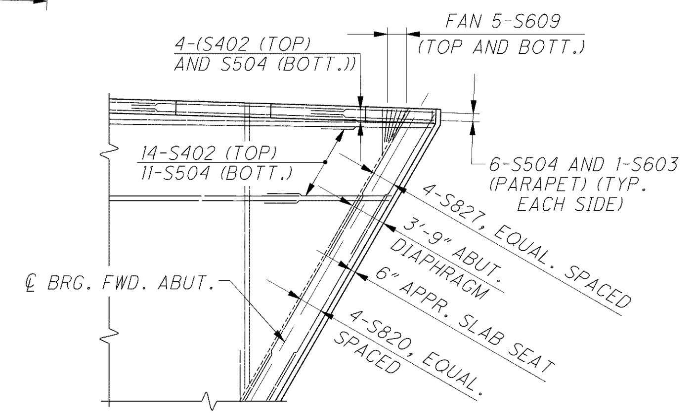
SLAB DETAIL 'B'
