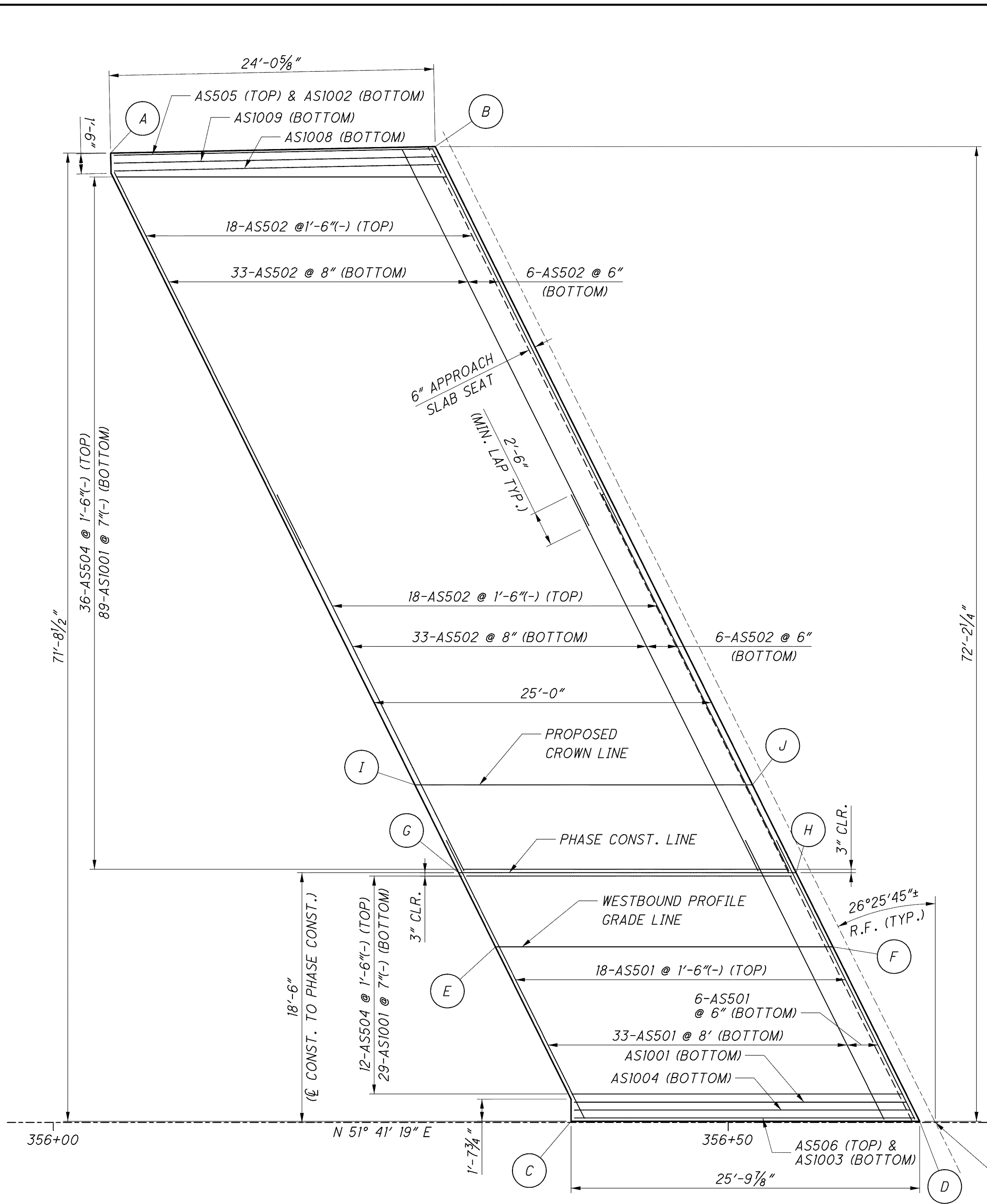
REAR APPROACH SLAB PLAN
