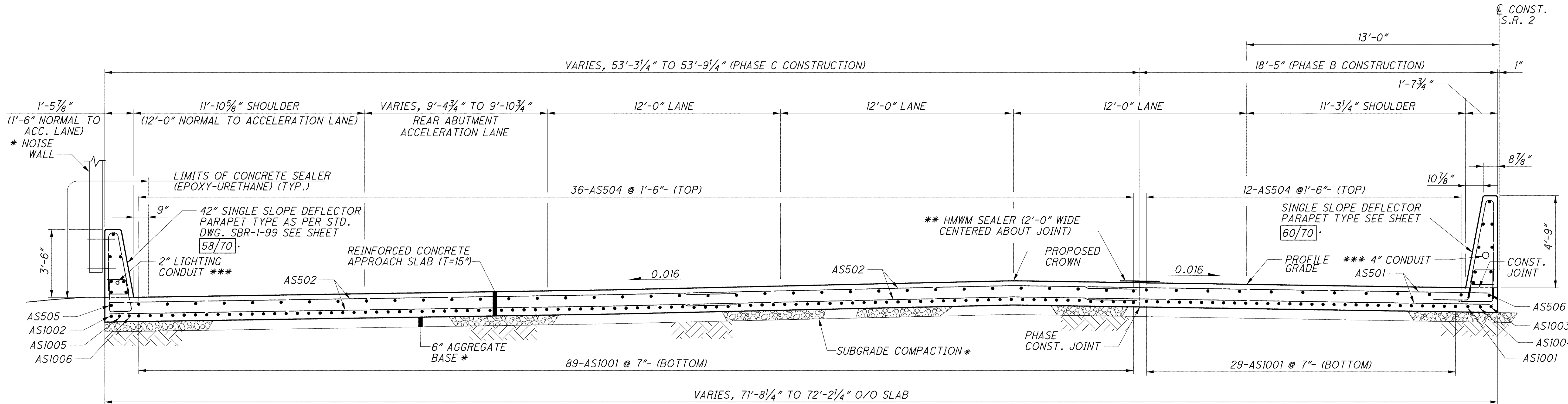
APPROACH SLAB TYPICAL SECTION WESTBOUND REAR
