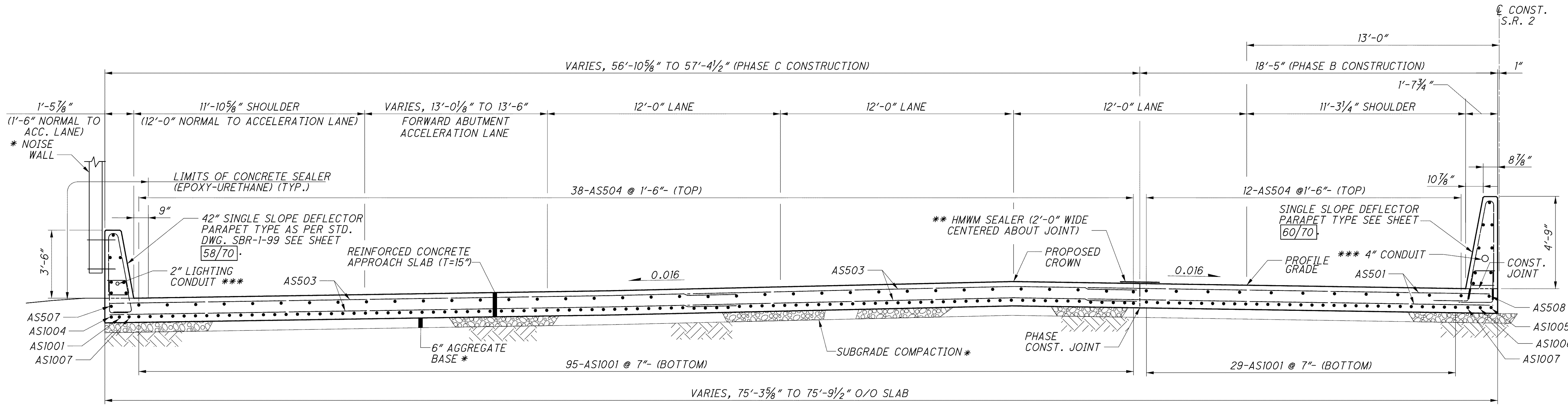
APPROACH SLAB TYPICAL SECTION WESTBOUND FORWARD
