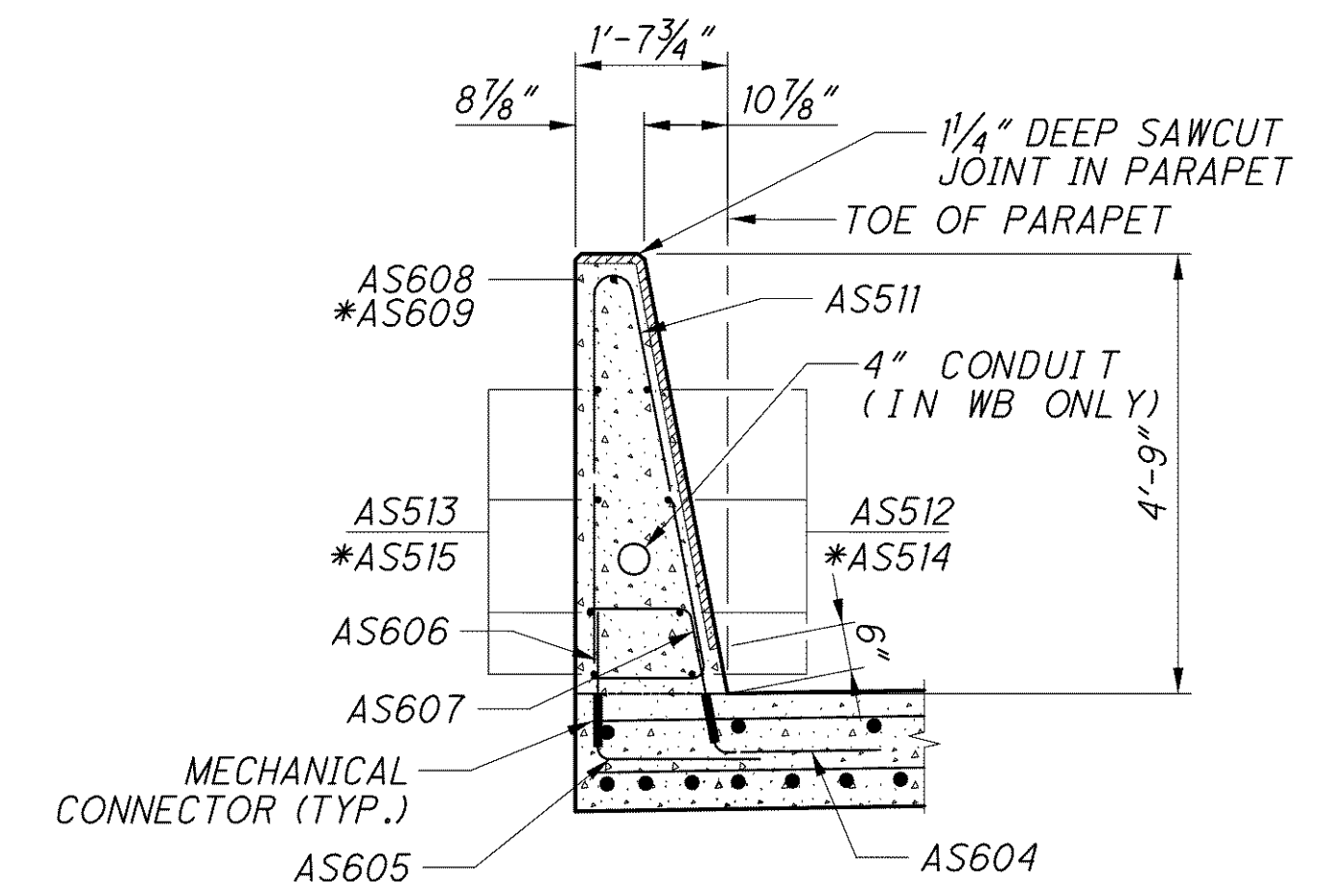
SECTION B-B
