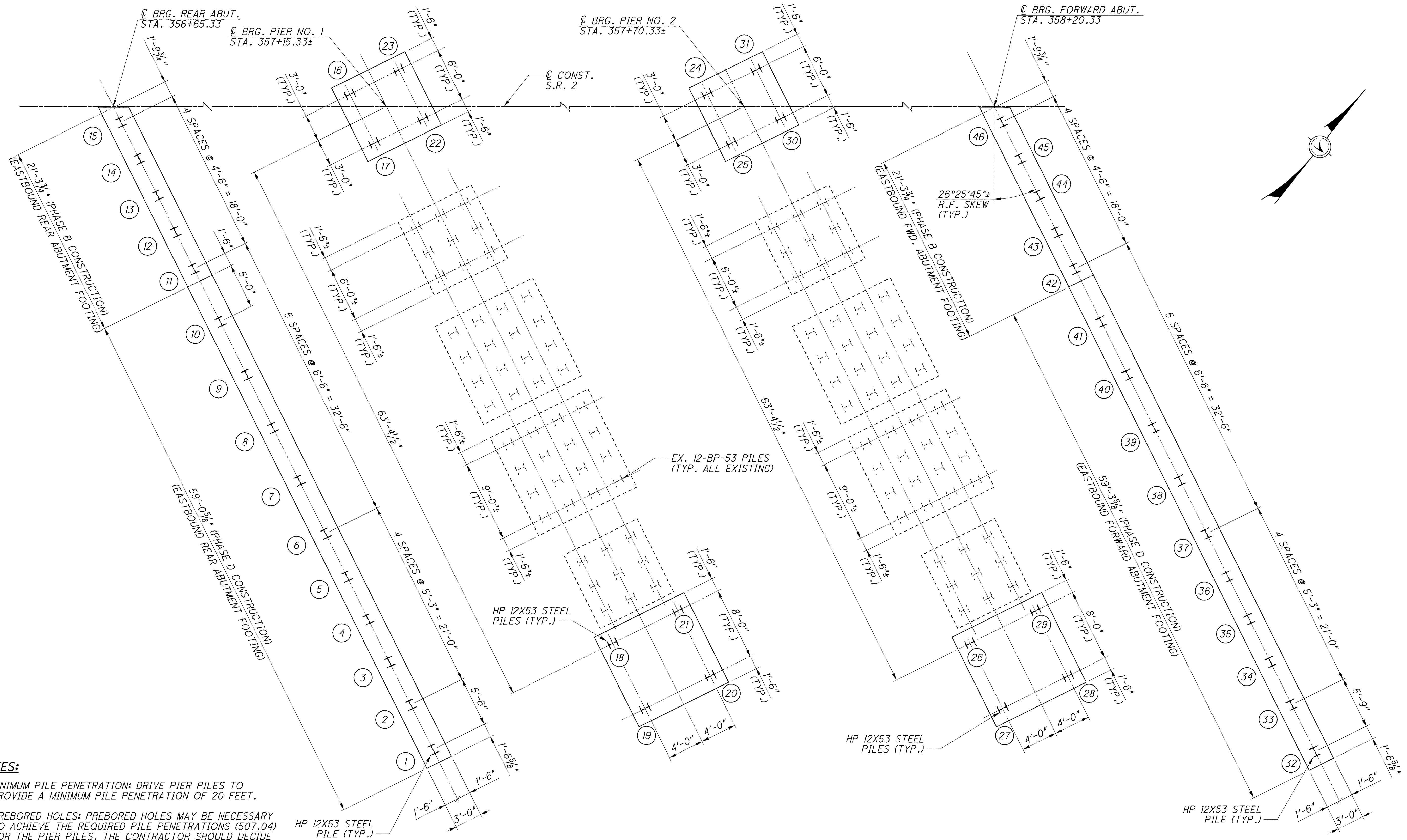
FOUNDATION PLAN (EASTBOUND)
