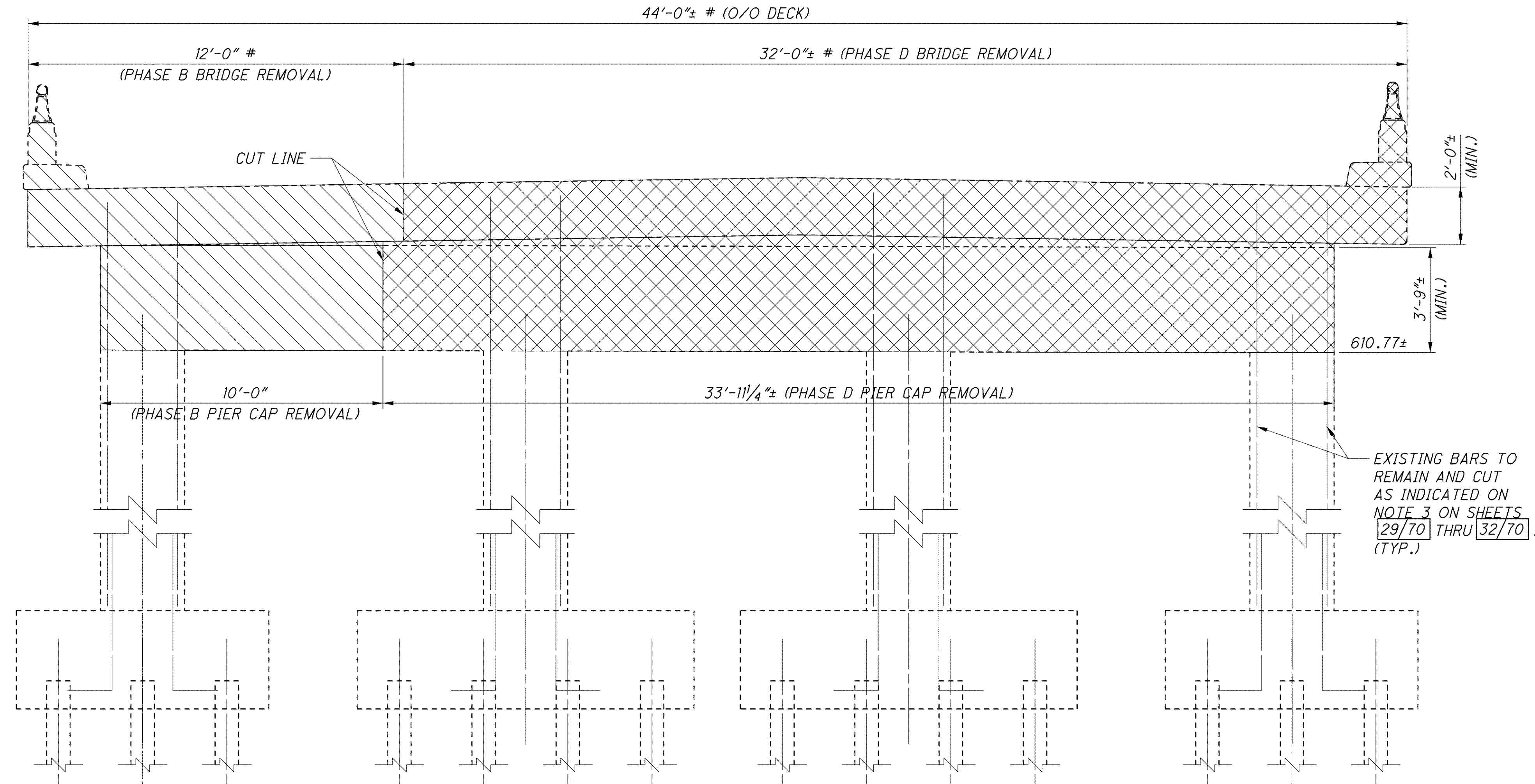
ELEVATION EASTBOUND SHOWN WESTBOUND SIMILAR
