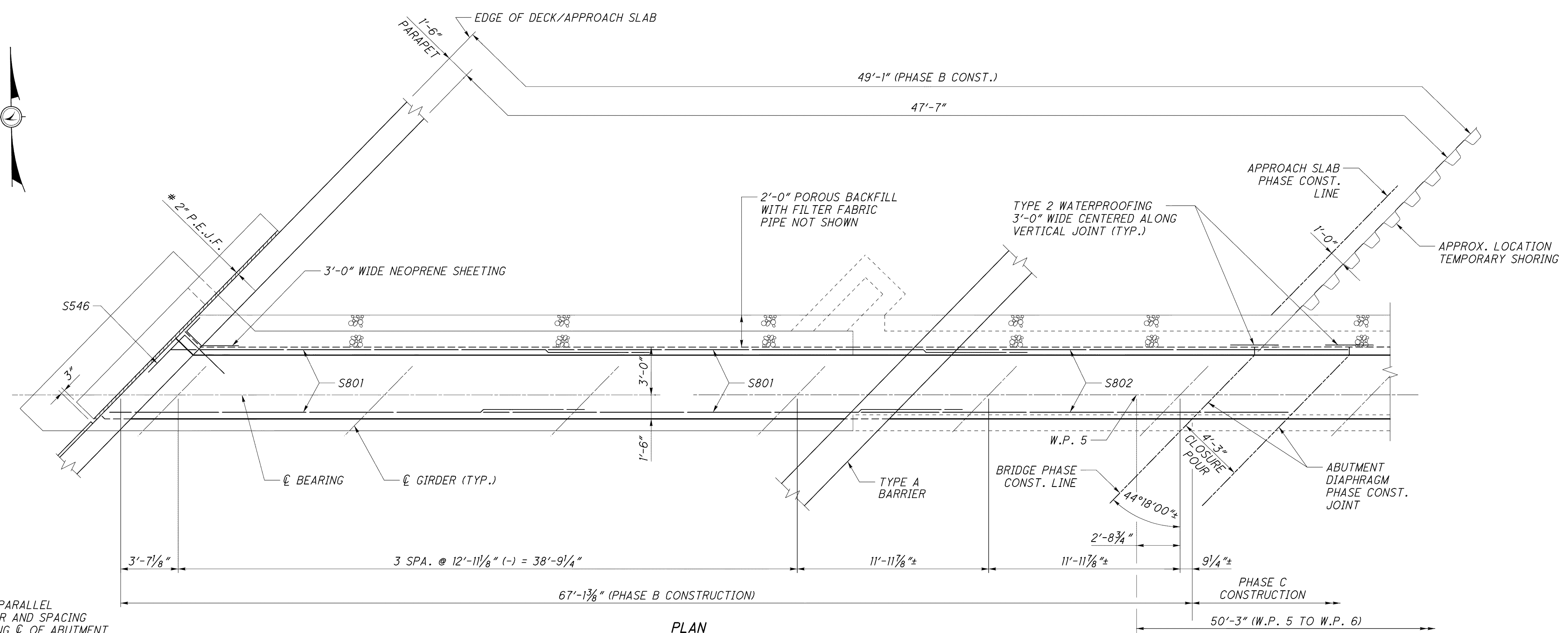
PLAN (LEFT FORWARD ABUTMENT DIAPHRAGM) (TOP 4-#8 BARS, BOTTOM 5-#8 BARS, & SHEAR REINFORCING NOT SHOWN FOR CLARITY)
