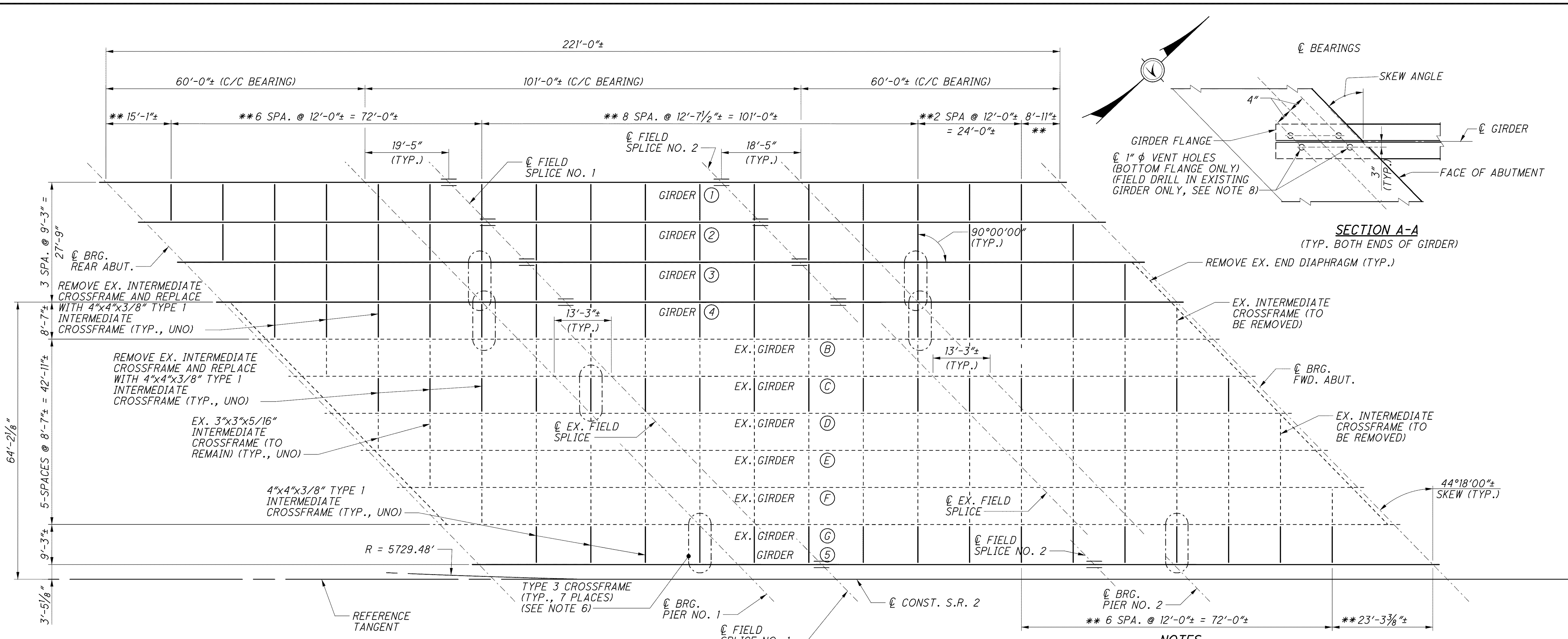
FRAMING PLAN (LEFT STRUCTURE)
