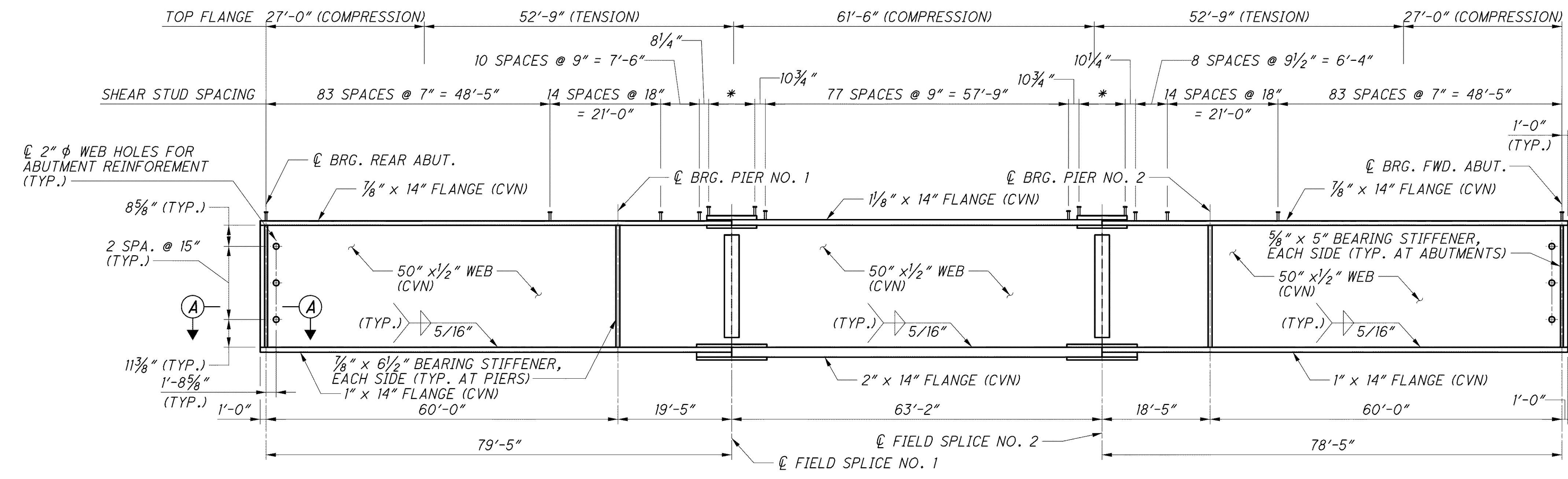
PROPOSED GIRDER ELEVATION
