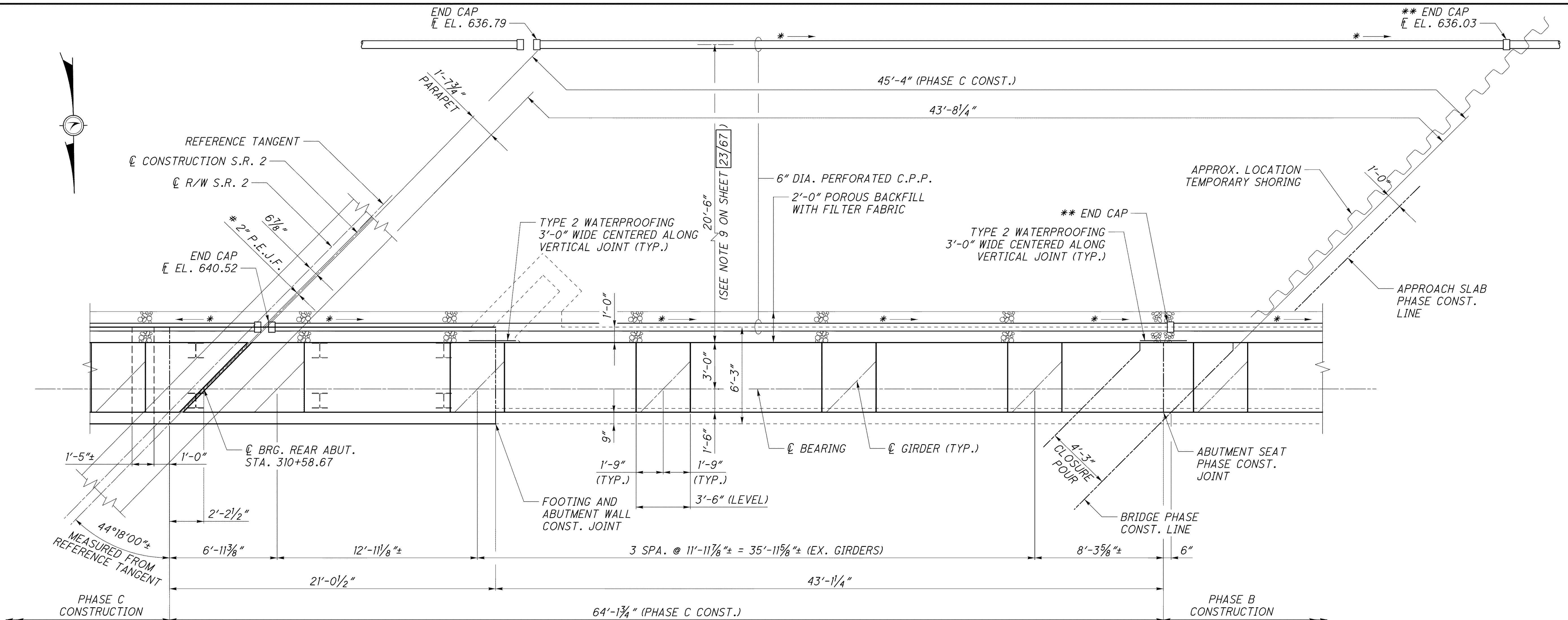
PLAN (LEFT REAR ABUTMENT)
