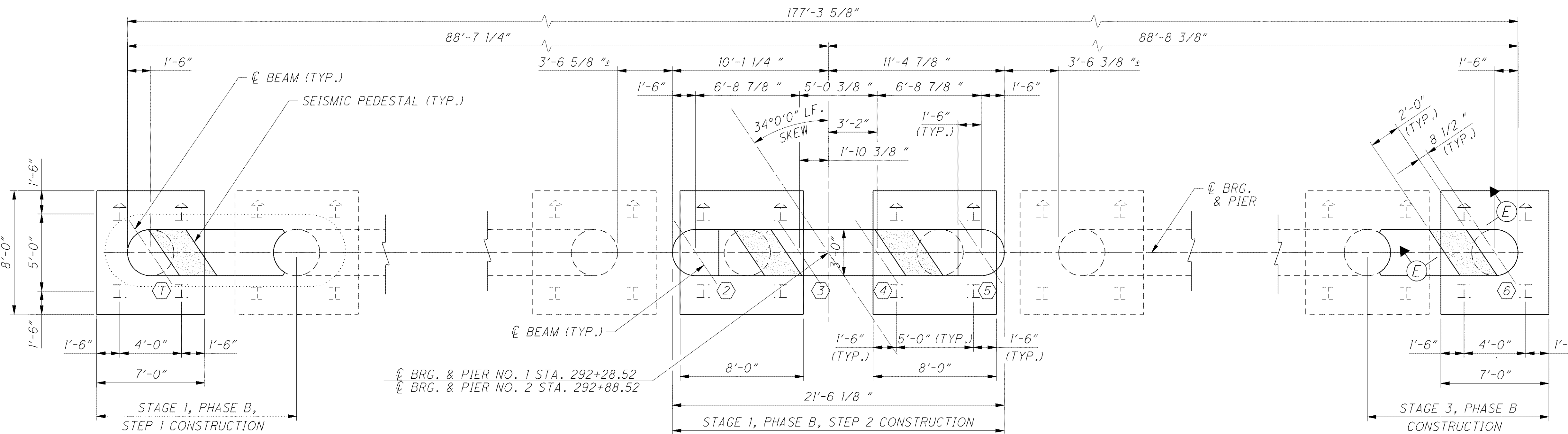
PLAN (PIER 1 SHOWN, PIER 2 SIMILAR)
