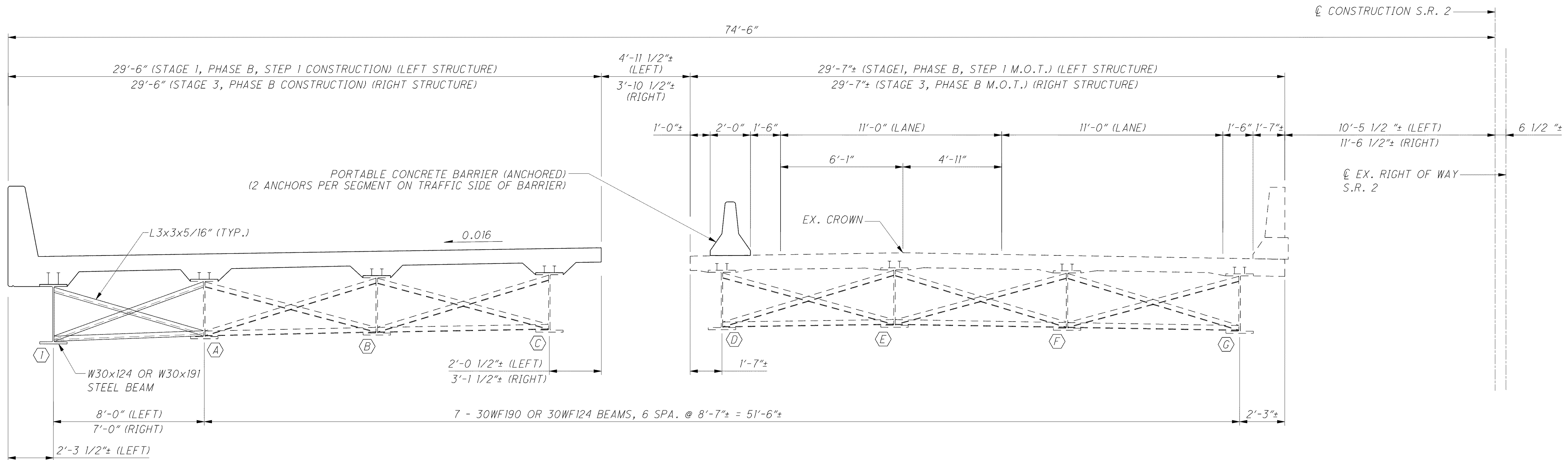
STAGE 1, PHASE B, STEP 1 CONSTRUCTION (LEFT STRUCTURE) STAGE 1, PHASE B, STEP 1 MAINTENANCE OF TRAFFIC (LEFT STRUCTURE) STAGE 3, PHASE B CONSTRUCTION (RIGHT STRUCTURE) STAGE 3, PHASE B MAINTENANCE OF TRAFFIC (RIGHT STRUCTURE)
